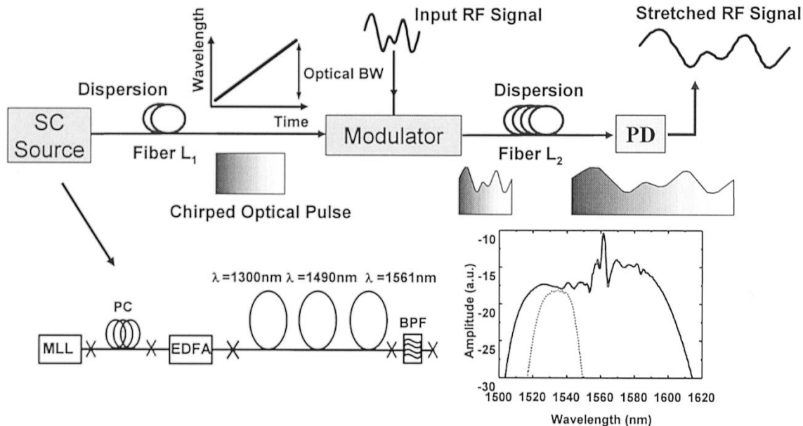
Fig. 3. Functional block diagram for the photonic time-stretch predecessor. A linearly chirped optical pulse is obtained by dispersing an ultra-short ultra-wide-band pulse (the SC). Time-to-wavelength mapping is achieved when this pulse is intensity-modulated by the electrical signal. The inset is the diagram of a three-stage SC generation. SC: Supercontinuum. PD: Photodetector.
