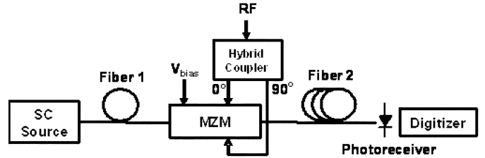
Fig. 9. Block diagram of the SSB-modulated photonic time-stretched A/D converter. The hybrid coupler provides 90^\circ RF phase shift between its two output ports. MZM: Mach-Zehnder modulator. SC: Supercontinuum.
