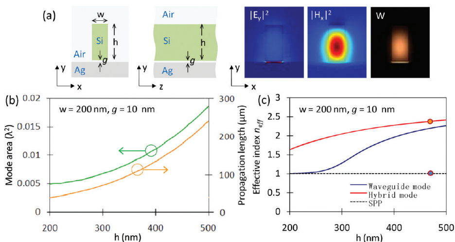
Figure 2. (a) Cross section of the hybrid plasmonic waveguide consisting of a rectangular silicon waveguide ( w/h = 200/470 nm) and silver substrate separated by an air gap ( g = 10 nm), and the distributions of electric field |E_y|^2 , magnetic field |H_x|^2 , and EM energy density W for the fundamental hybrid mode at 200 THz propagating along the z -axis. (b) Mode area A_m and the propagation length L_m of the hybrid mode as a function of the waveguide height h . (c) The h dependence of effective index n_{\text{eff}} for the hybrid mode (red curve), bare silicon waveguide mode (blue curve), and bare SPP mode (dotted curve).
