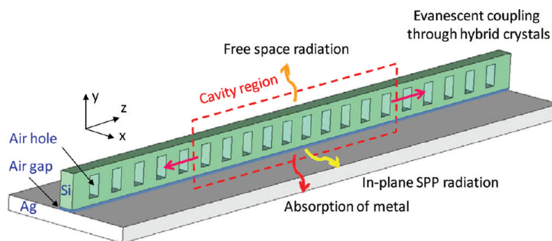
Figure 1. Schematic of the proposed hybrid photonic–plasmonic crystal nanocavity consisting of 10 lattice periods with parabolic variation of lattice constant in the cavity region. The photon loss channels of the hybrid crystal cavity modes include free space radiation, in-plane SPP radiation, evanescent coupling through hybrid crystals, and absorption of metal.
