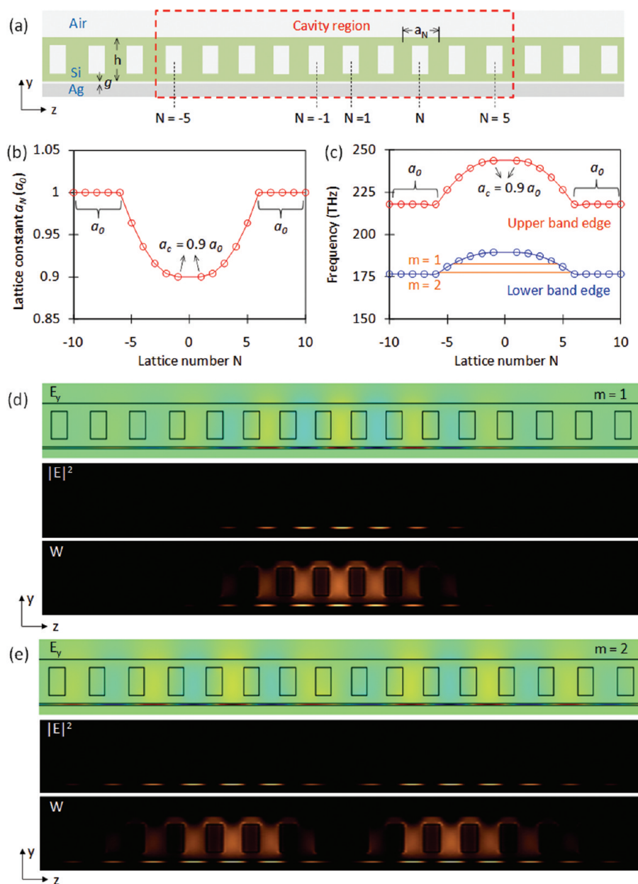
Figure 4. (a) Schematic of the hybrid crystal nanocavity consisting of 10 lattice periods in the cavity region. (b) Lattice constant a_N along the waveguide as a parabolic function of the lattice number N from a_0 to a_c = 0.9a_0 . (c) Lower and upper band-edge frequencies along the waveguide. The created acceptor-type cavity supports two eigenmodes ( m = 1 and m = 2 ) inside the mode gap. The corresponding field distributions ( E_y , |E|^2 , and W ) for the two eigenmodes (d) m = 1 and (e) m = 2 of hybrid crystal cavity with g = 10 nm.
