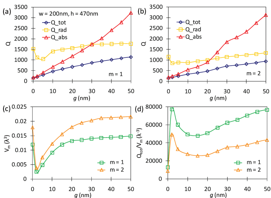
Figure 5. Dependences of quality factors Q_{tot} , Q_{rad} , and Q_{abs} on the gap separation g with w = 200 nm and h = 470 nm for the two eigenmodes (a) m = 1 and (b) m = 2 . (c) Mode volume V_m and (d) Q_{tot}/V_m ratio as a function of air gap g for the two eigenmodes.
