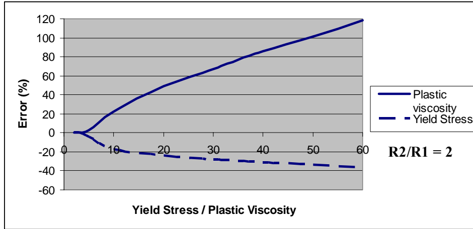
Figure 2.11 Influence of ratio of yield stress to plastic viscosity on errors due to neglecting the dead zone for rotation speed 10 rpm to 60 rpm (Koehler, 2004)
