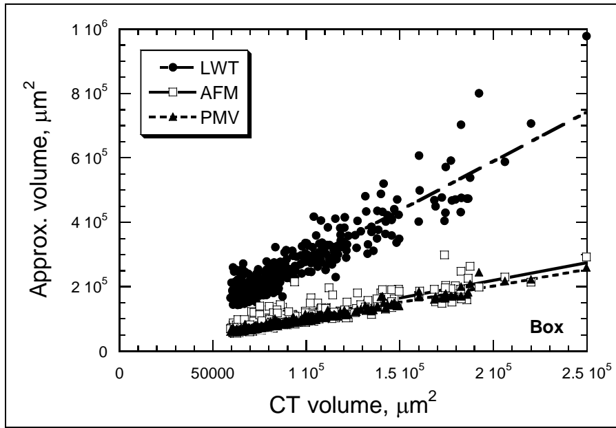
Figure 6.15 Box volume estimates for the microfinest (Taylor et al., 2005)
