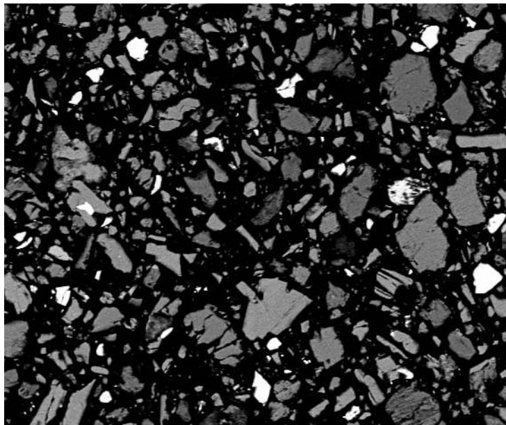
Figure 6.12 Grayscale SEM image of microfine aggregates at 500x magnification
