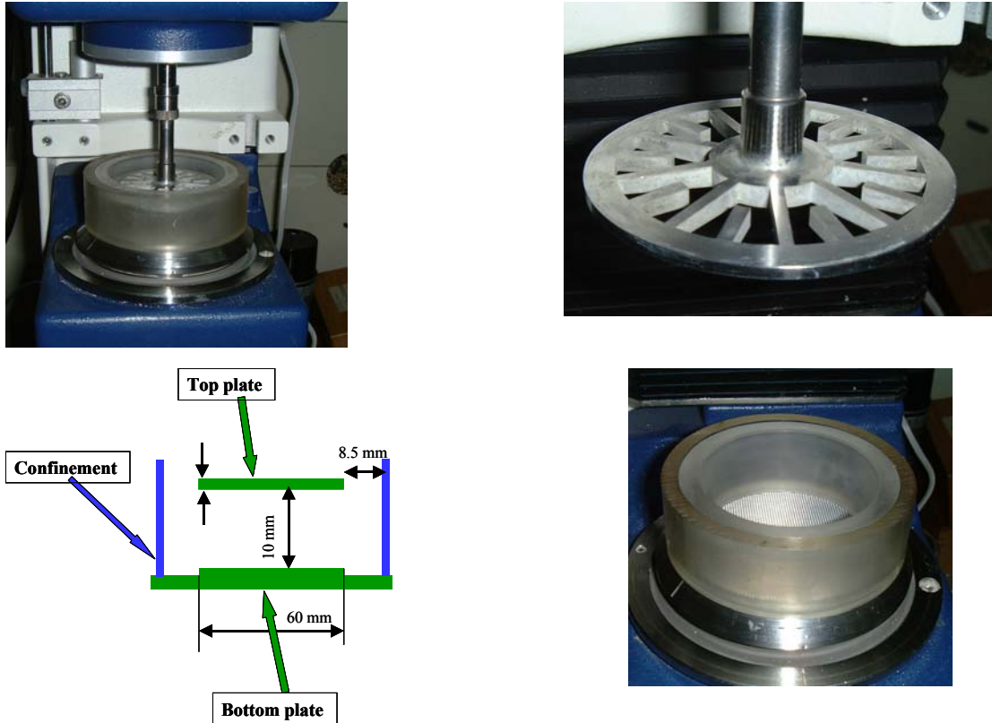
Figure 5.9 The parallel plate mortar rheometer (clockwise from top left: overall view, top plate, bottom plate and confinement ring, schematic showing dimensions)
