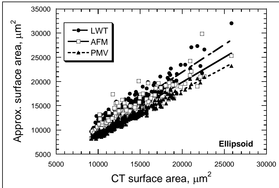
Figure 6.16 Ellipsoid surface area estimates for the microfinest (Taylor et al., 2005)
