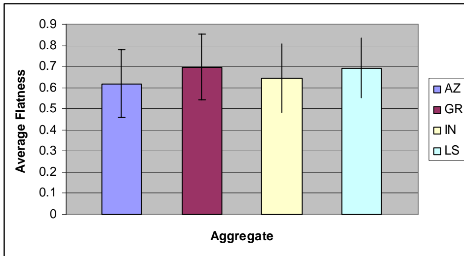
Figure 6.3 Individual and average flatness values for the particles of the four different coarse aggregates scanned
