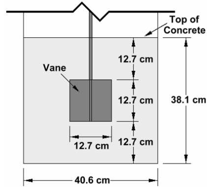
Figure 5.6 ICAR rheometer positioned over its container and the dimensions of the rheometer
