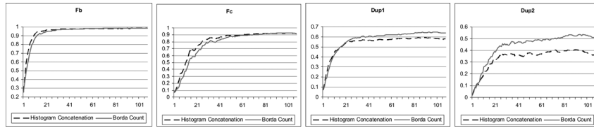
Fig. 6. Comparison between histogram concatenation and Borda count combination with 108 LBP histograms on the FERET database.
