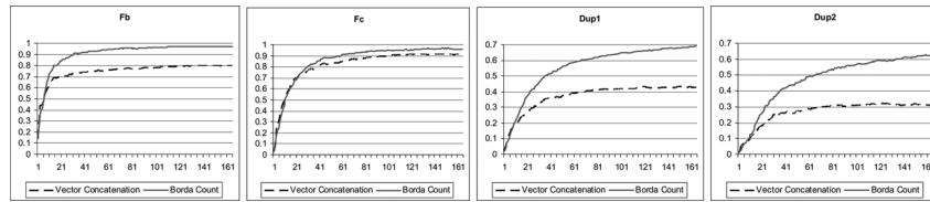
Fig. 5. Comparison between feature vector concatenation and Borda count combination with 165 Gabor jets on the FERET database.
