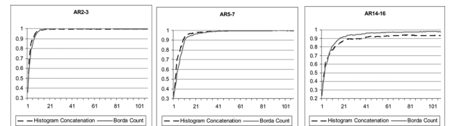
Fig. 8. Comparison between histogram concatenation and Borda count combination with 108 LBP histograms on the AR database.
