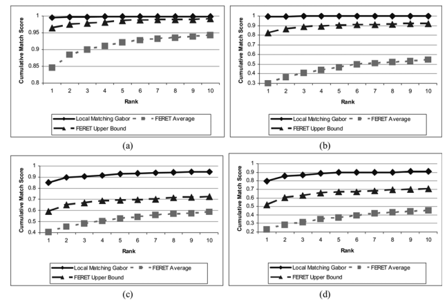
Fig. 9. Cumulative match curves on FERET (a) Fb, (b) Fc, (c) Dup1, and (d) Dup2 probes. FERET average and upper bound performance is estimated from the printouts of [35, Figs. 7 and 8].
