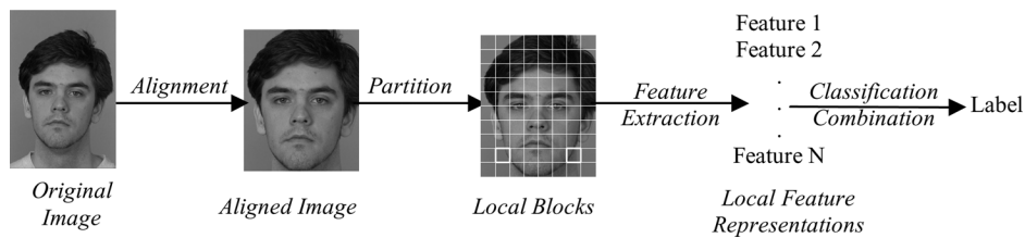
Fig. 1. Diagram of local matching face recognition.
