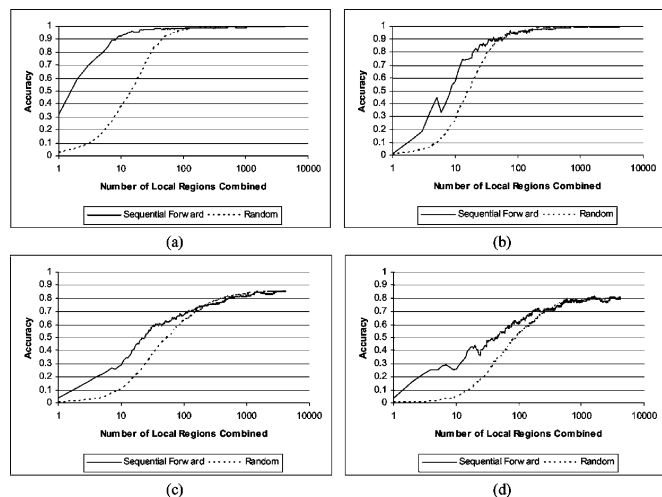
Fig. 11. Accuracies on (a) Fb probes, (b) Fc probes, (c) Dup1 probes, and (d) Dup2 probes with respect to the number of Gabor jets combined.
