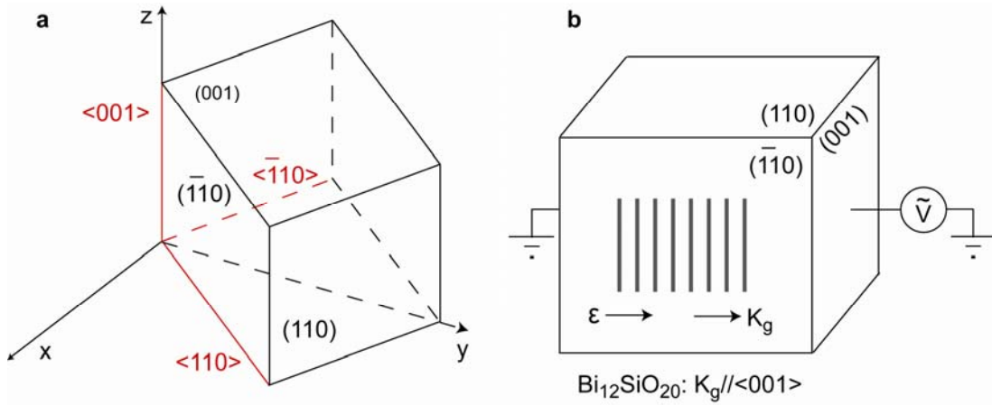
Figure 2.1. Bi_{12}SiO_{20} photorefractive crystal. (a) Crystal orientation and its crystallographic axes x , y , and z . (b) A high voltage square wave electric field is applied on the two (0\ 0\ 1) faces of the crystal to enhance the wave mixing and holographic recording efficiencies. Both the signal and pump light beams are incident on the (-1\ 1\ 0) face.
