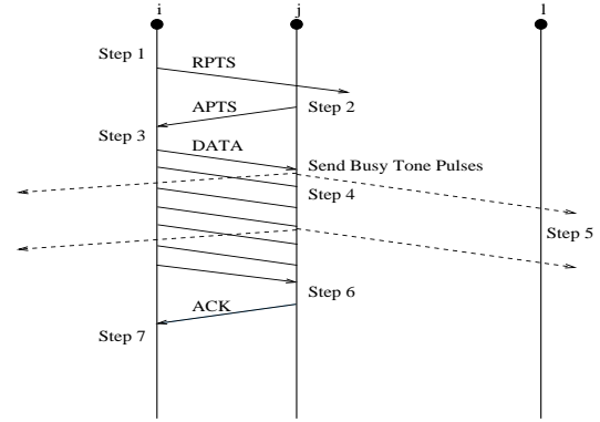
Fig. 3. PCMA protocol steps
