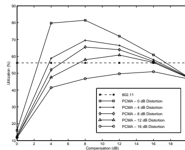
Fig. 11. Throughput for different amounts of busy tone distortion with varying compensations in a 1000x1000 meter network
