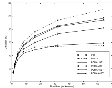
Fig. 4. 100 nodes in a 1000x1000 meter network with 100 flows each sending 2 KB packets, and a connectivity range of 250 meters
