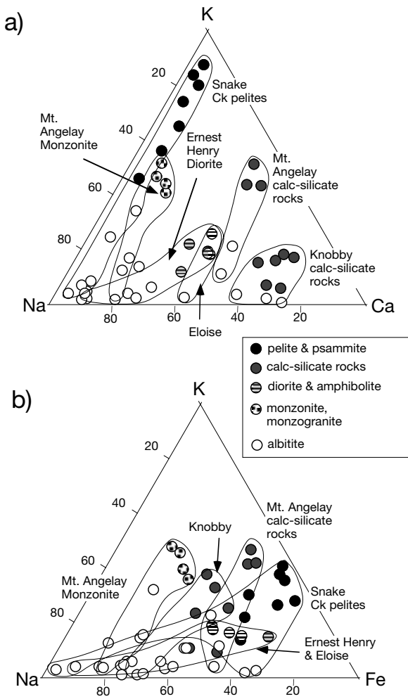
FIG. 11. Summary triangular diagrams for albitization, calculated using raw oxide data (i.e., assumes total mass changes are negligible; see Fig. 10) from Table 5 and other unpublished data. a. CaO-Na 2 O-K 2 O. b. Na 2 O-K 2 O-Fe 2 O 3 (all Fe determined as Fe 2 O 3 ). Outlined fields enclose least altered rocks (darker dots) and their albitized equivalents (white dots) from various locations, as indicated. Some rocks show little relative decrease in Ca or Fe, but others show depletions in all of K, Ca, and Fe, and all rocks show an increase in Na/K ratio with albitization.
