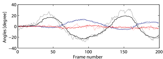
Fig. 17 Comparison between the estimated poses and the ground truth. Dashed: estimations by our method; Solid: the ground truth. Black: yaw; Red: pitch; Blue: roll.
