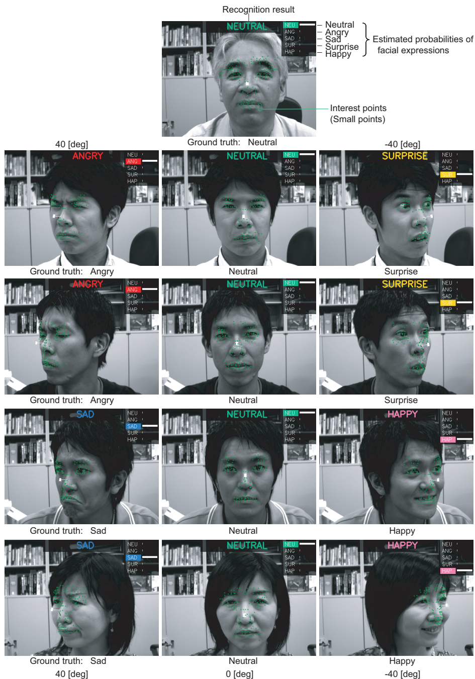
Fig. 9 Some estimation results of facial poses and expressions with fixed-pose dataset (Horizontal): The expression in the upper part of each image denotes the recognized result. The width of each bar in the upper right part of each image denotes the estimated probability of each facial expression, P(e_t|z_{1:t}) . Small points on each face denote interest points.
