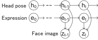
Fig. 5 Dynamic Bayesian Network for head poses, facial expressions, and face images.
