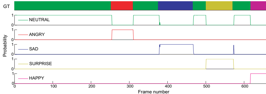
(b) Ground truth (top) and recognition results (others) of facial expression: The probability of correct expression is remarkably higher than that of other expressions.
