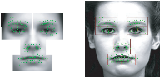
Fig. 14 Left: Example of set of interest points defined in the average facial part images \bar{g}_{e,p} that are learned with the Cohn-Kanade DFAT-504 database. Right: The set of interest points \mathcal{P} generated by projecting the average facial part image into the initial frame, or the training image for neutral expression g_{j,NEU} , of a target subject.
