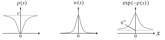
Fig. 6 Shape of robust function \rho(x) , weight function w(x) = (d\rho(x)/dx)/x , and \exp(-\rho(x)) , similar to the likelihood function.
