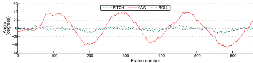
(c) Estimation results of facial pose (horizontal axis equals that of (b)): Facial poses are estimated with enough accuracy to detect three cycles of head shake movement (red solid line).
