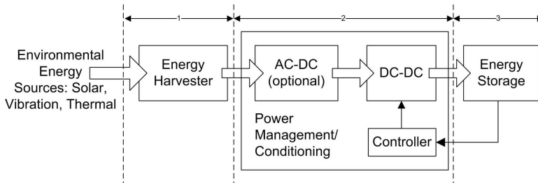
Fig. 10. General block diagram representation of energy harvesting system unit
