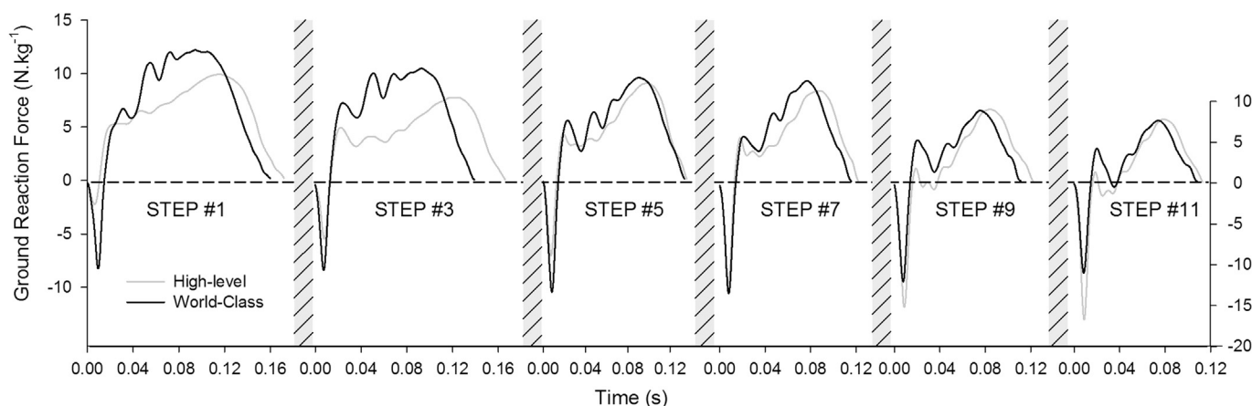
Fig. 2. – Comparison of instantaneous horizontal ground reaction force during the support phases of the 1st, 3rd, 5th, 7th, 9th and 11th steps of a 40-m sprint between a world-class sprinter (100-m best time of 9.95 s, black lines) and a high-level sprinter (100-m best time of 10.60 s, grey lines). Only odd-numbered steps are shown for clarity reasons.
