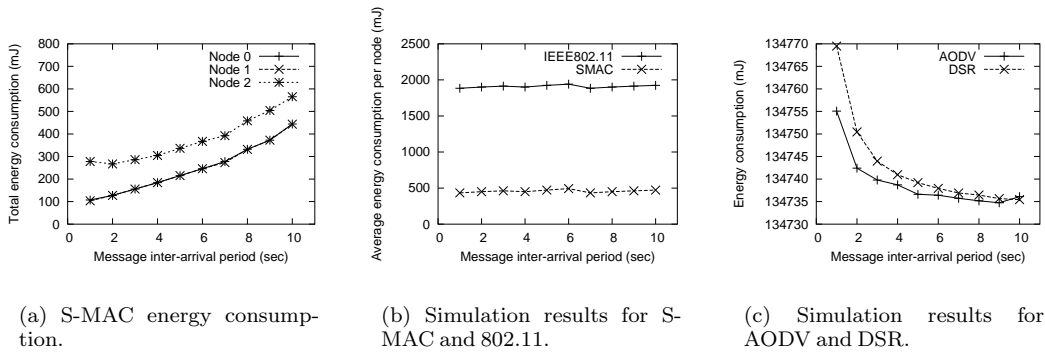
Figure 3. Simulations results using instrumented GloMoSim/QualNet.
