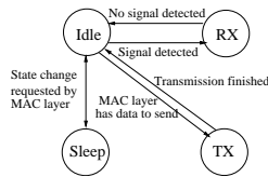
Figure 1. State diagram for radio modes
