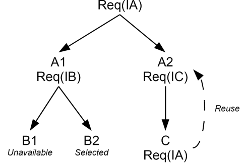
Figure 4: Component selection search tree for interface IA
