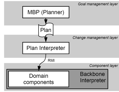
Figure 5: Implementation entities
