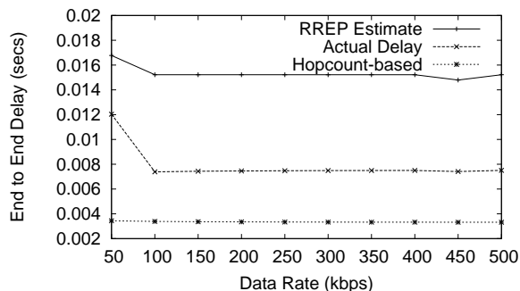
Figure 3: End to End Delay Estimation of the data packets. RREP overestimates end-to-end delay because of inter-flow interference. The hopcount-based approach underestimates the delay since it does not account for intra-flow interference.
