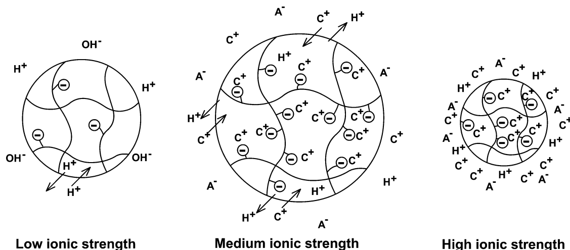
Fig. 5 The swelling of a pH-sensitive hydrogel as a function of the ionic strength. ( A^- , C^+ mean anion and cation respectively).
