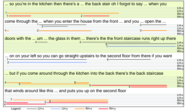
Fig. 3. Oscillation-scored Transcript
