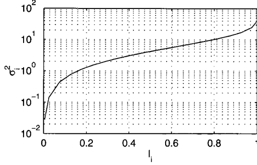
Fig. 7. Mapping between the parameters \sigma_i^2 and I_i .
