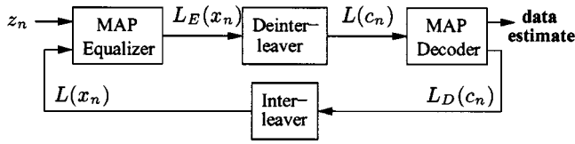
Fig. 3. A receiver performing turbo equalization.
