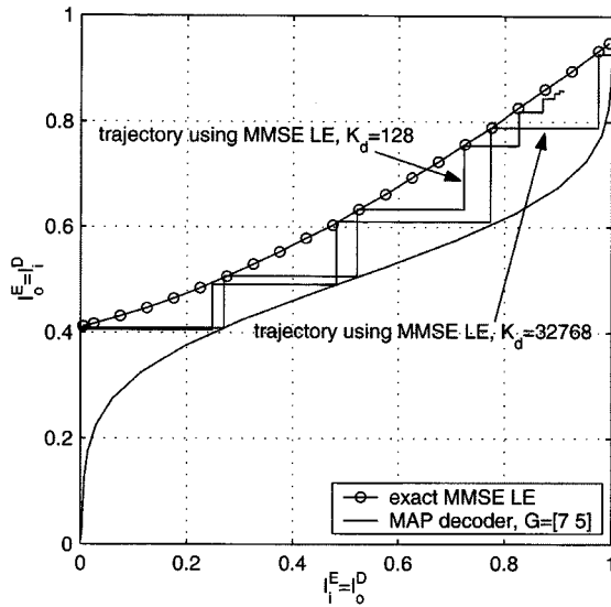
Fig. 16. Receiver EXIT charts with traces of a receiver using linear MMSE equalization at two block lengths K_d .
