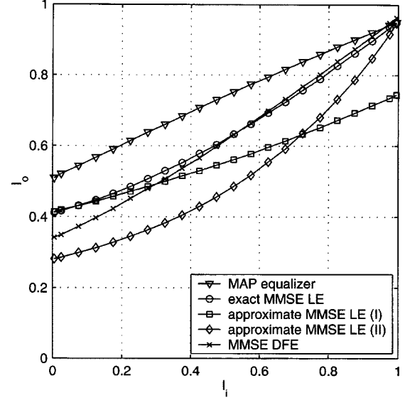
Fig. 9. EXIT charts of the equalizer at 4-dB SNR.
