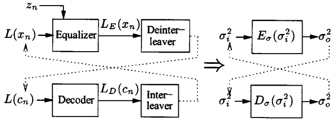
Fig. 6. Model for analysis of the iterative receiver algorithm.
