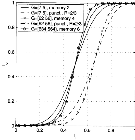
Fig. 8. EXIT charts of a map decoder.
