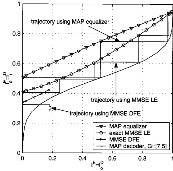
Fig. 14. Receiver EXIT charts with traces of iterative algorithms.
