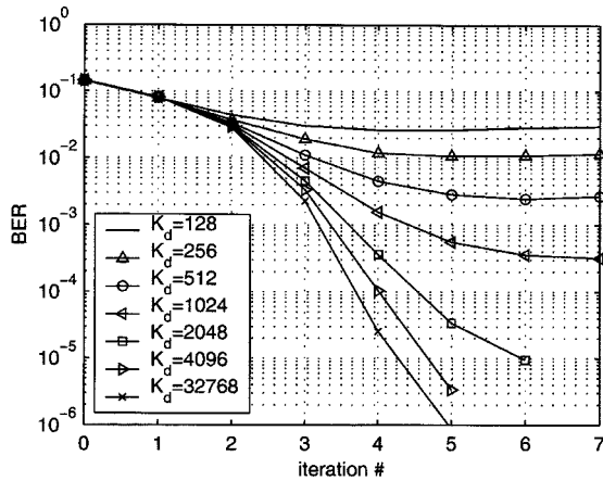
Fig. 17. BER of the receiver at 4 dB E_s/N_0 using exact MMSE linear equalization for several iterations and block lengths K_d .
