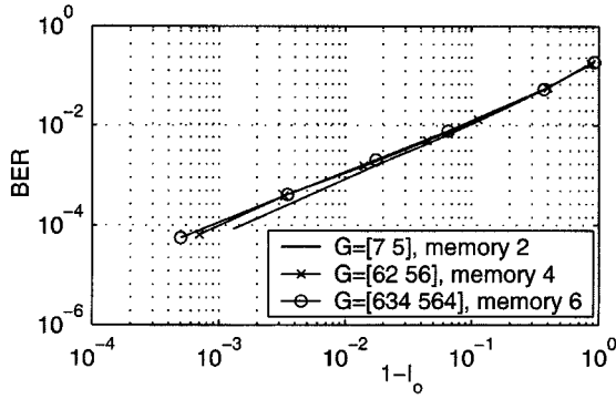
Fig. 10. Information BER of MAP decoding as a function of I_o .
