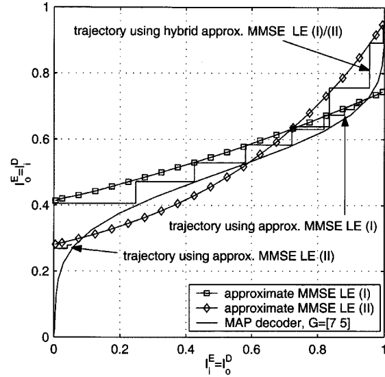
Fig. 15. Receiver EXIT charts with traces of a receiver using hybrid linear MMSE equalization.
