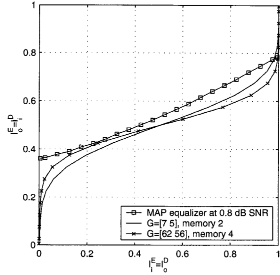
Fig. 12. Receiver EXIT chart at 0.8 dB E_s/N_0 for various codes.
