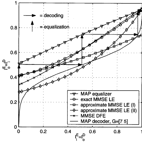
Fig. 11. Receiver EXIT chart at 4 dB E_s/N_0 .
