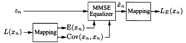
Fig. 4. A SISO equalizer based on MMSE equalization.
