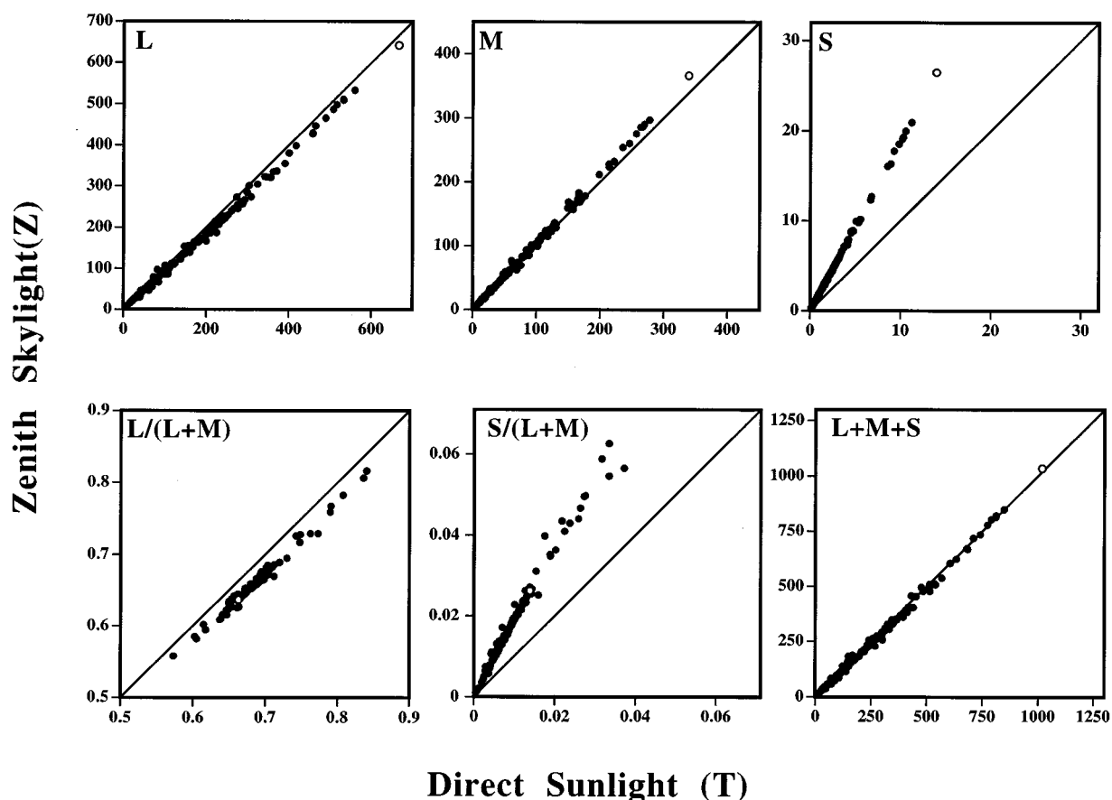
Fig. 1. Excitation of the L , M , and S cones (top three plots) and the exclusive excitation of the chromatic and luminance mechanisms along the L/(L + M) , S/(L + M) , and L + M + S axes (bottom three plots) from each of the 170 objects from Vrhel et al. 23 under illuminants T [direct sunlight (abscissa)] and Z [zenith skylight (ordinate)]. The open circles represent the object of unit uniform spectral reflectance.
