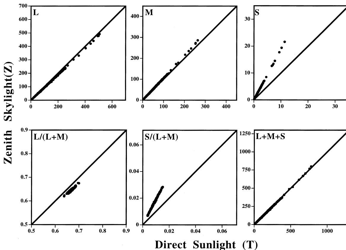
Fig. 2. Excitation of the L , M , and S cones (top three plots) and the exclusive excitation of the chromatic and luminance mechanisms along the L/(L + M) , S/(L + M) , and L + M + S axes (bottom three plots) from each of the 335 natural formations from Krinov 31 under illuminants T (abscissa) and Z (ordinate).
