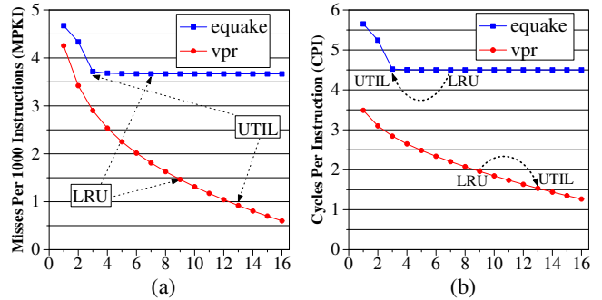
Figure 1. (a) MPKI and (b) CPI as cache size is varied when vpr and quake are executed separately. The horizontal axis shows the number of ways allocated from a 16-way 1MB cache (remaining ways are turned off).
