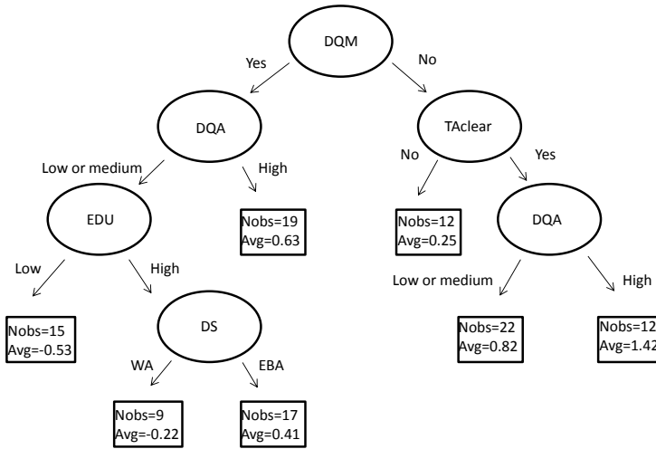
Figure 3.3: A regression tree for the confidence level of decision makers on their decision outcomes with MSE=0.089 .
