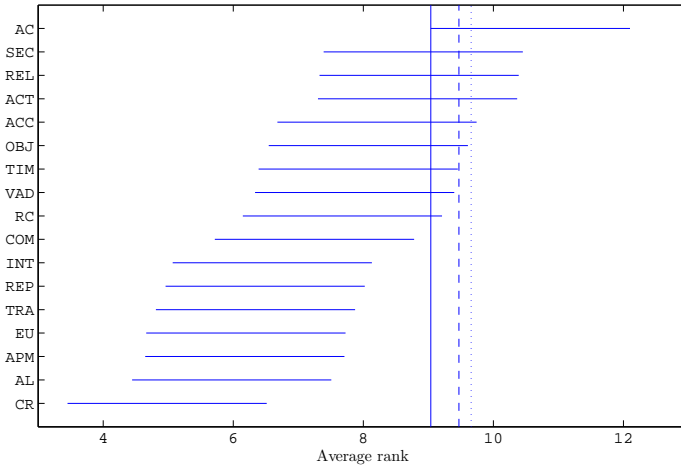
Figure 2.5: Bonferroni-Dunn plot of the relative importance of the DQ dimensions in financial institutions
