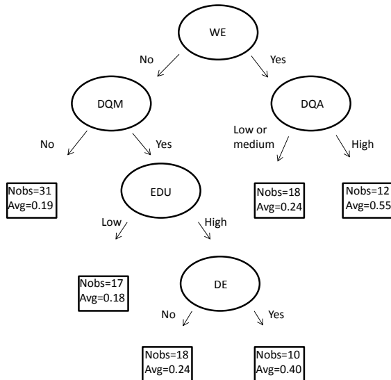
Figure 3.4: A regression tree for the decision time measured in minutes with MSE=0.0118 .
