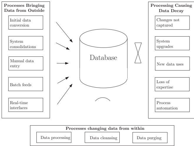
Figure 2.3: Different data inputting and manipulating processes, adopted from Maydanchik [86]
