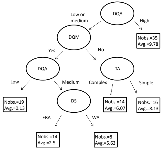
Figure 3.2: A regression tree for the decision accuracy (DA) with MSE=0.5715 . The minimum score is zero and the maximum is 10.
