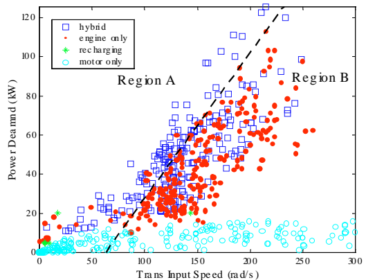
Figure 6: Operating points of DP optimization over UDDSHDV cycle
