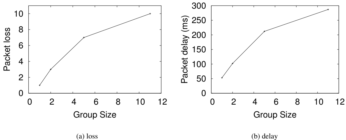
Figure 13: Packet loss and delay in different group size experiments
