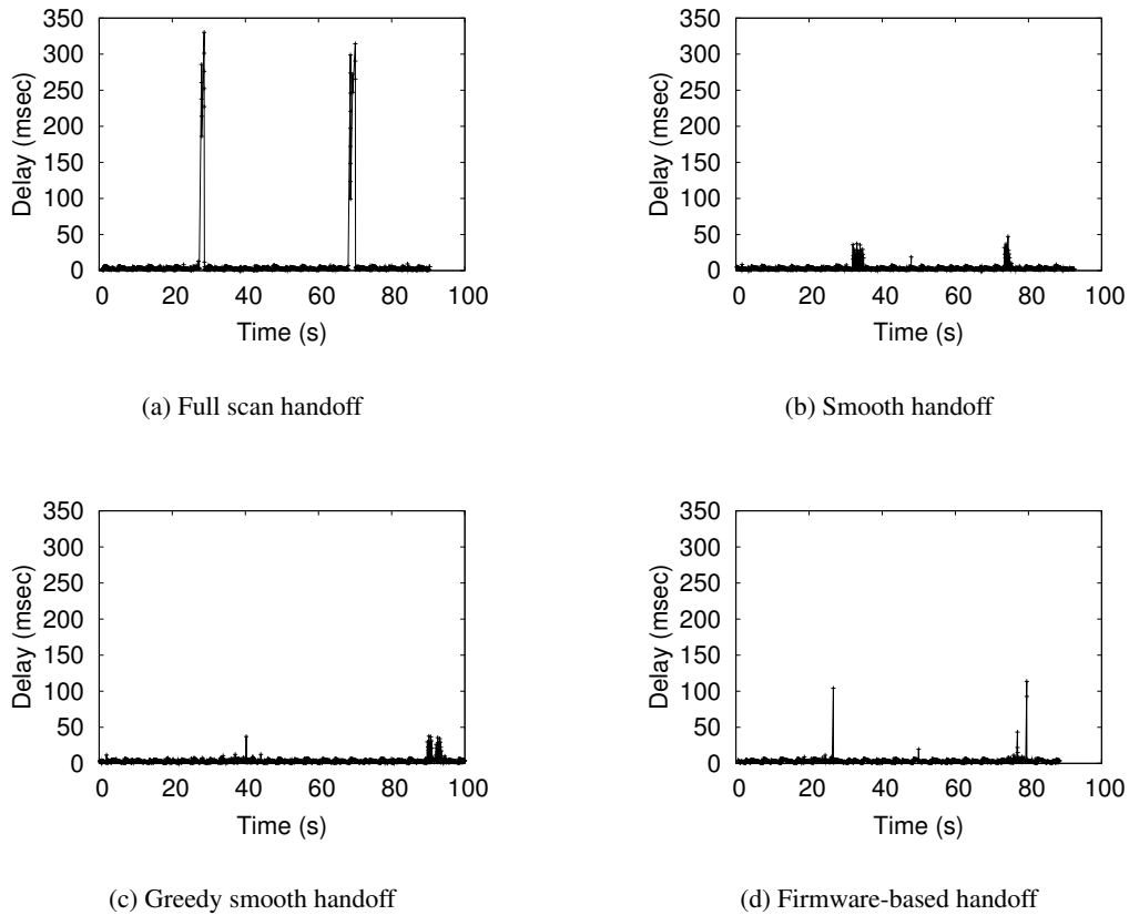
Figure 8: Packet delay in different handoff schemes (channel group size is 1 in smooth handoff and greed smooth handoff schemes)
