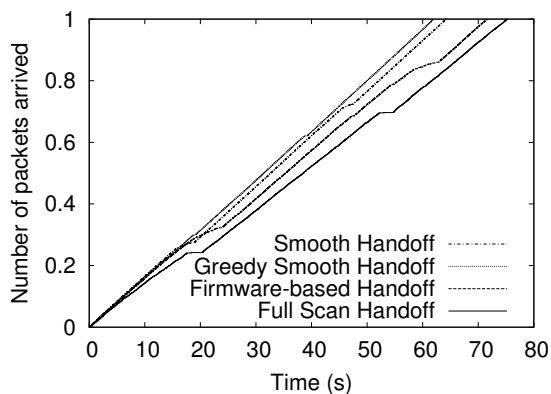
Figure 11: Upload experiment
