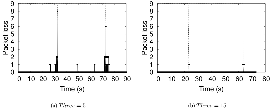
Figure 12: Packet loss in different threshold experiments
