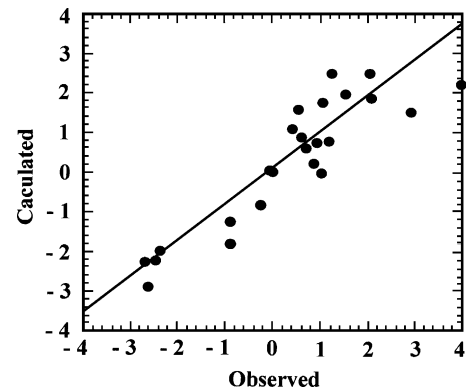
Fig. 4. Rationalisation of the effects of mutations on the aggregation rates of peptides and proteins. The observed experimental aggregation rates of a variety of short peptides or natively unfolded proteins, including amylin, amyloid \beta -peptide, tau and \alpha -synuclein (see Table 1 for a summary of the diseases with which these are associated) are shown plotted against rates calculated from an algorithm derived from extensive mutational studies of the protein acylphosphatase. The numbers are the natural logarithms of the changes in aggregation rate. Such a correlation argues strongly for a common mechanism for amyloid formation and provides a platform both to predict the effects of natural mutations and to design polypeptides with altered aggregation properties. From [66].
