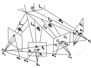
Figure 2. The quadrilinear constraint in terms of pairs of intersecting planes.
