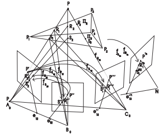
Figure 3. Invariant projective depth using n uncalibrated cameras.
