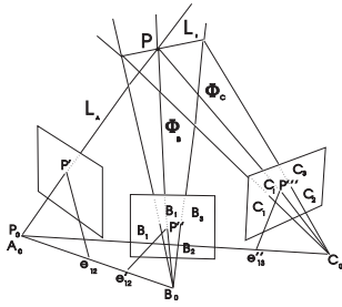
Figure 1. The trilinear constraint in terms of intersecting lines and planes.
