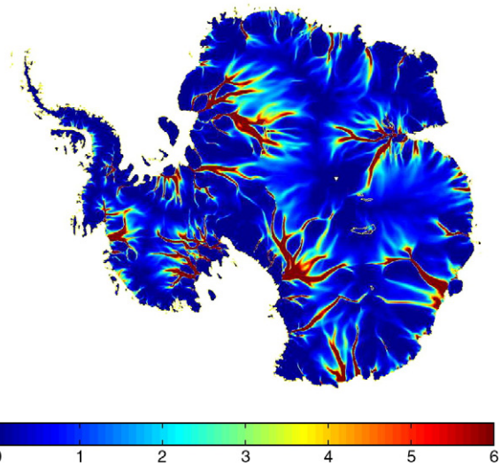
Fig. 5. Subglacial water flux ( 10^3 \text{ m}^2 \text{ year}^{-1} ) based on the mean basal melt rate displayed in Fig. 4A. Values are truncated at 6 \times 10^3 \text{ m}^2 \text{ year}^{-1} .
