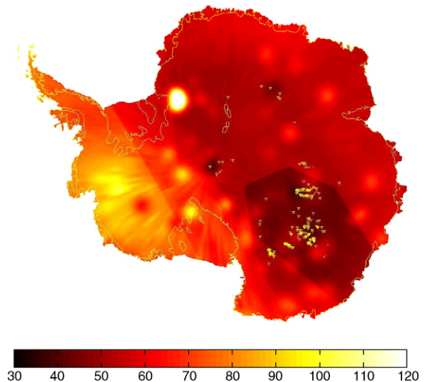
Fig. 2. Geothermal heat flow (GHF) based on a combination of Shapiro and Ritzwoller (2004) and Pollard et al. (2005) and corrected for basal temperature gradients from ice cores as well as the distribution of different subglacial lake types using (19)–(22).
