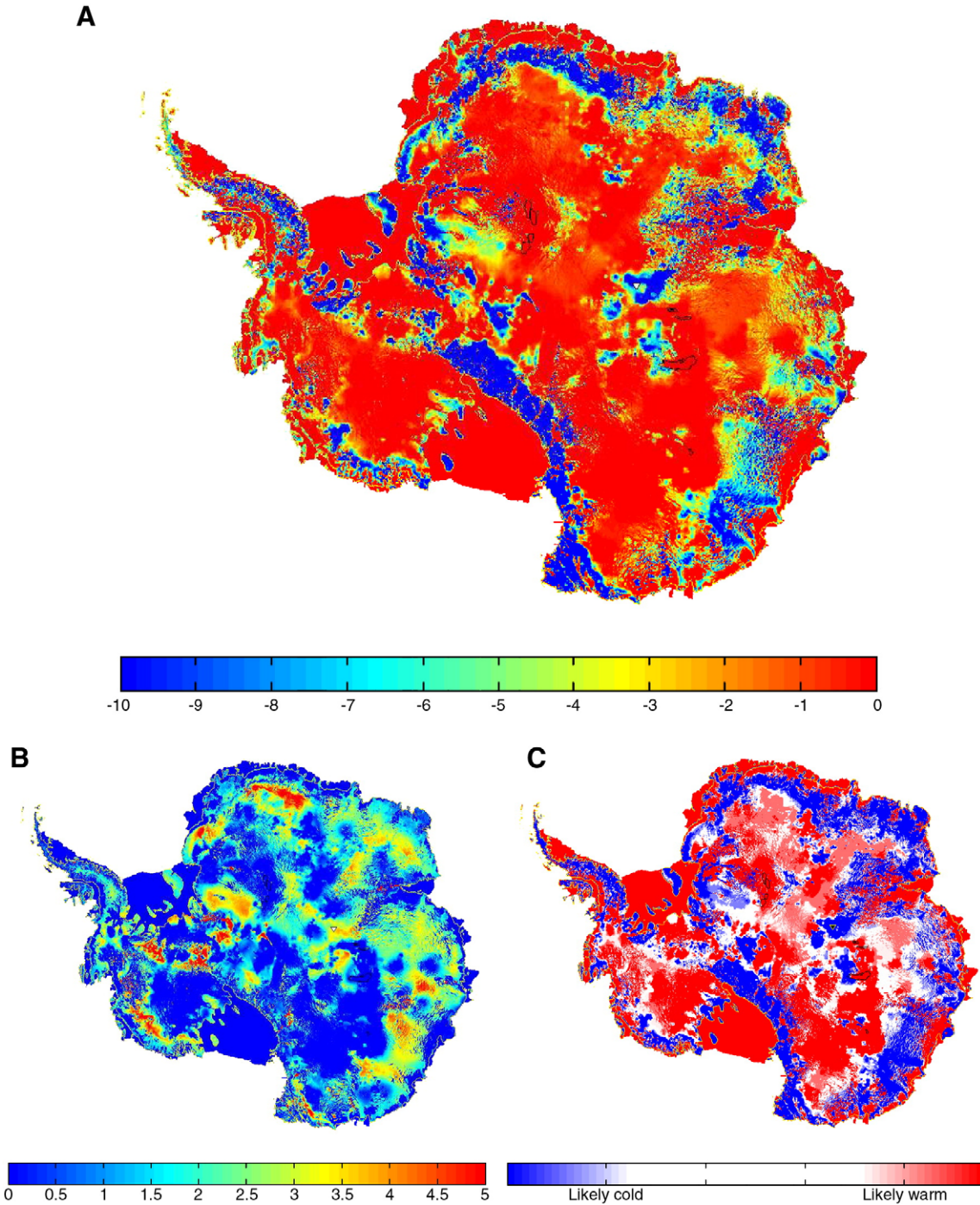
Fig. 3. (A) Mean basal temperature ( ^{\circ}\text{C} , corrected for pressure melting and truncated at -10^{\circ}\text{C} ); (B) standard deviation ( ^{\circ}\text{C} ) for the 24 sensitivity experiments; and (C) likelihood of cold and warm bed (scale from 0 (cold-based in all experiments) to 24 (warm-based in all experiments)). The triangle shows the position of Dome Argus, where a new deep ice core drilling is planned.
