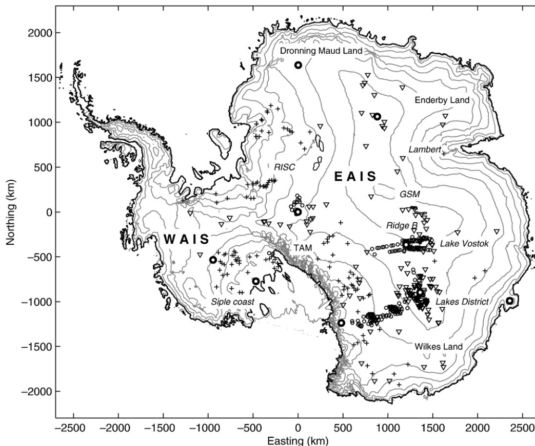
Fig. 1. Surface topography (Bamber et al., 2009) of the Antarctic ice sheet with RES identified large subglacial lakes (black lines), definite ( \nabla ) subglacial lakes (Siebert et al., 2005a; Carter et al., 2007; Popov and Masolov, 2007), fuzzy ( \circ ) lakes (Carter et al., 2007) and active ( + ) lakes (Smith et al., 2009). The large dots show the position of the deep drill sites where the temperature profile is measured. The present-day grounding line is shown by a black line. WAIS = West Antarctic Ice Sheet; EAIS = East Antarctic Ice Sheet; TAM = Transantarctic Mountains; RISC = Recovery Ice Stream Catchment; GSM = Gamburtsev Subglacial Mountains.
