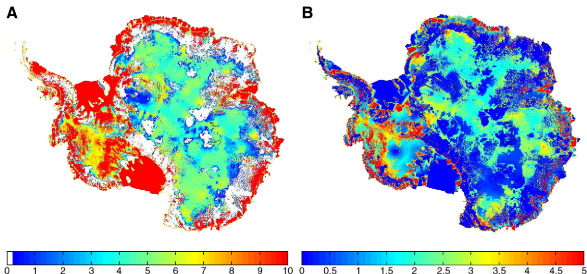
Fig. 4. (A) Mean basal melting rate (truncated at 10 \text{ mm year}^{-1} ) and (B) standard deviation ( \text{mm year}^{-1} ) for the 24 sensitivity experiments.
