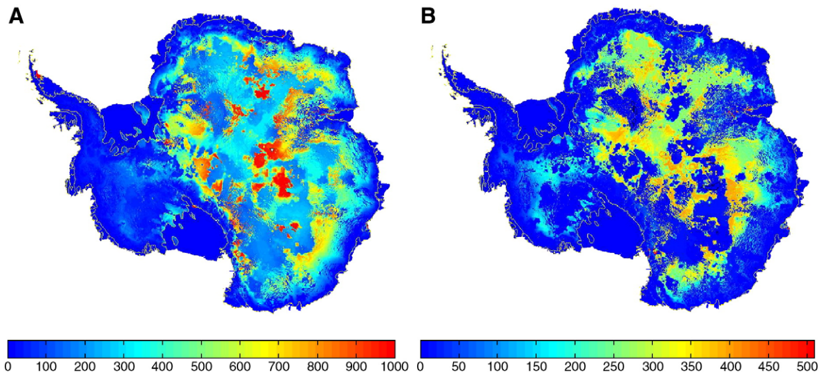
Fig. 7. (A) Mean ice age at 98% depth ( 10^3 year) and (B) standard deviation ( 10^3 years) for the 24 sensitivity experiments.
