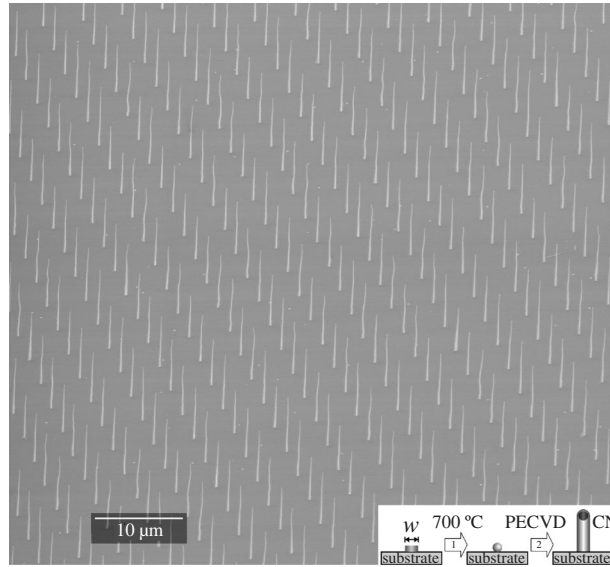
Figure 4. CNTs grown on a support at precisely defined positions using plasma-enhanced CVD. (Reproduced with permission from Teo et al. (2003).) The nanotubes were grown from 100 nm wide dots of 7 nm thick Ni catalyst.
