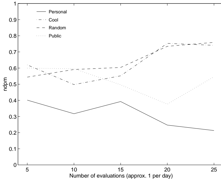
Figure 6: For each source, distance between user’s rankings and its ideal ranking, averaged over all users at each evaluation point.
