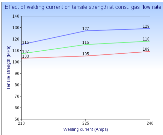
Fig. 2 Welding current Vs Tensile strength
