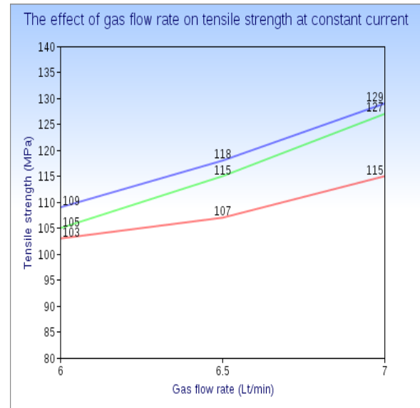
Fig. 3 Gas flow rate Vs Tensile strength
