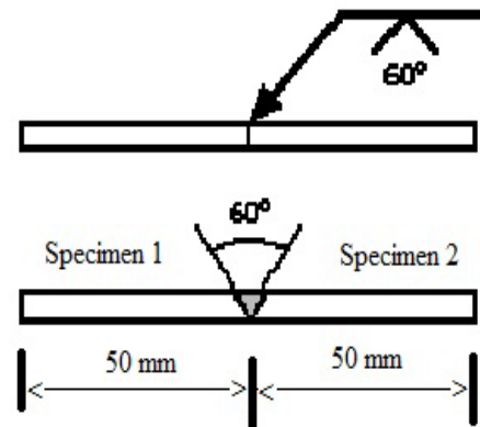
Fig. 1 V-groove b/w specimens for welding
