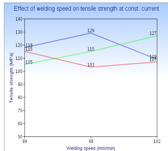
Fig. 4 Welding speed Vs Tensile strength
