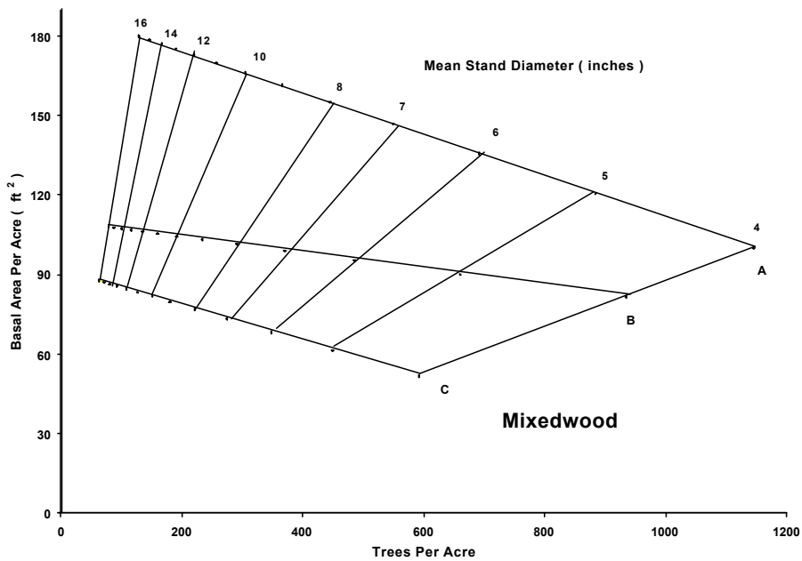
Figure 3a and b.—Stocking charts for softwood and mixedwood stands based on trees in the main crown canopy. The A line is average maximum stocking. The B line is recommended minimum stocking for adequate growth response per acre. The C line defines the minimum amount of acceptable growing stock for a manageable stand (adapted from Figures 3 and 4, Solomon et al 1995).
