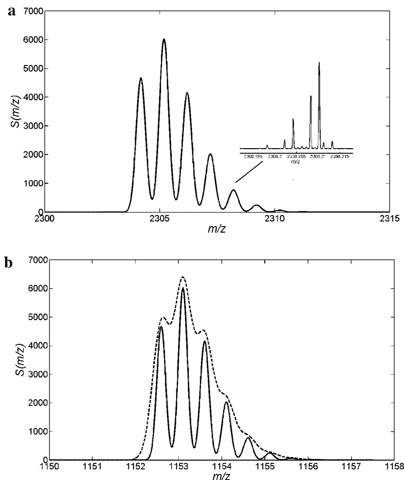
FIGURE 3. Theoretical signal shapes: The mean signals s_i of peptide STQVYGQDVWLPAETLDIR were calculated by the methods described in Rockwood, Orden, and Smith (1995) and Rockwood and Orden (1996). a: The singly charged distribution convoluted with a Gaussian of width 0.2 (full width at half maximum (FWHM) \approx 5,700 ). The inset shows the fine structure 5th isotopic group at a very high resolution, which is out of reach for standard instruments. b: The same peptide, but with charge z = 2 . The dashed line corresponds to FWHM \approx 3,000 and the solid line to FWHM \approx 5,700 .
