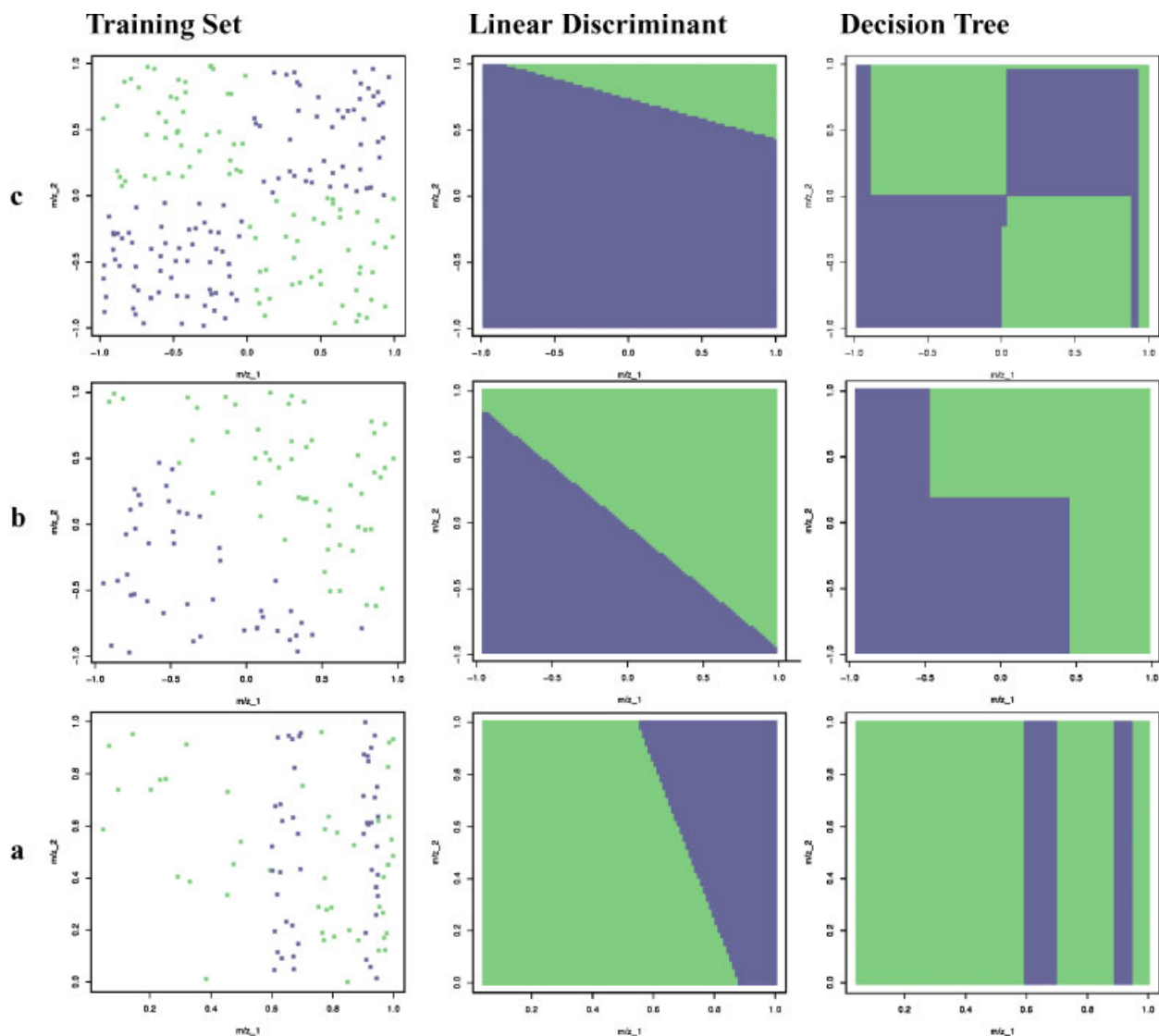
FIGURE 6. Three artificial learning problems with two features. Each problem (row) is represented by the training set (left column), the decision surface induced by a linear discriminant algorithm (middle), and the decision surface induced by a decision tree algorithm (right).
