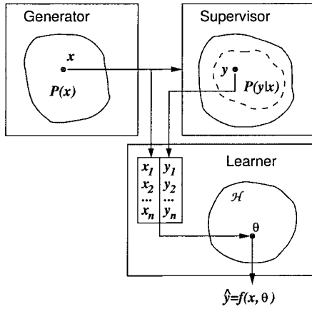
FIGURE 5. Classification as a supervised learning task. The training data are assumed to be drawn from an unknown probability distribution P(\mathbf{X}) and the class labels from P(Y|\mathbf{X}) . A learner builds a function that estimates the joint distribution P(\mathbf{X}, Y) to predict a class \hat{y} for a new instance x .
