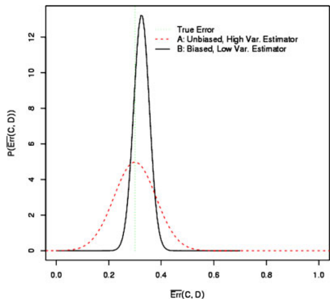
FIGURE 7. Examples of two hypothetical error estimators with different bias-variance profiles.
