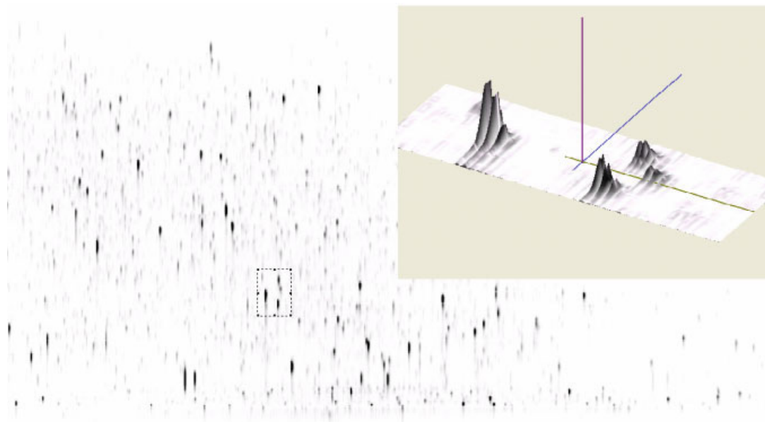
FIGURE 4. LC-MS data: this figure shows good-quality data, which contains very little noise. The elution time is along the vertical and m/z along the horizontal axis. The inset shows a 3-dimensional surface plot of the marked rectangle and reveals how four isotopic distributions smoothly elute over time. The images were produced by the MSight LC-MS viewer, freely available at http://www.expsy.org/MSight .
