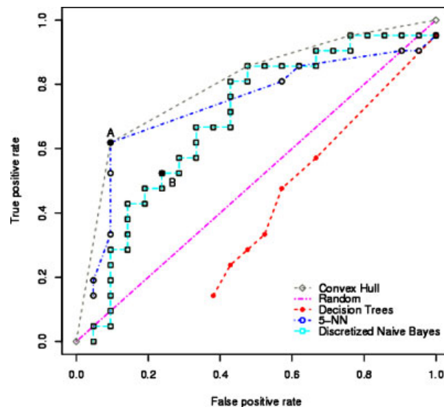
FIGURE 8. ROC curves of four different classifiers on a mass-spectrometry problem. For this specific problem, the convex hull contains discretized Naïve Bayes and 5-nearest-neighbors which can thus be optimal under certain conditions. Note that decision trees (DTs) fare worse than random, probably because their sequential variable selection mechanism assesses variables individually, in effect ignoring all interactions among peak intensities.
