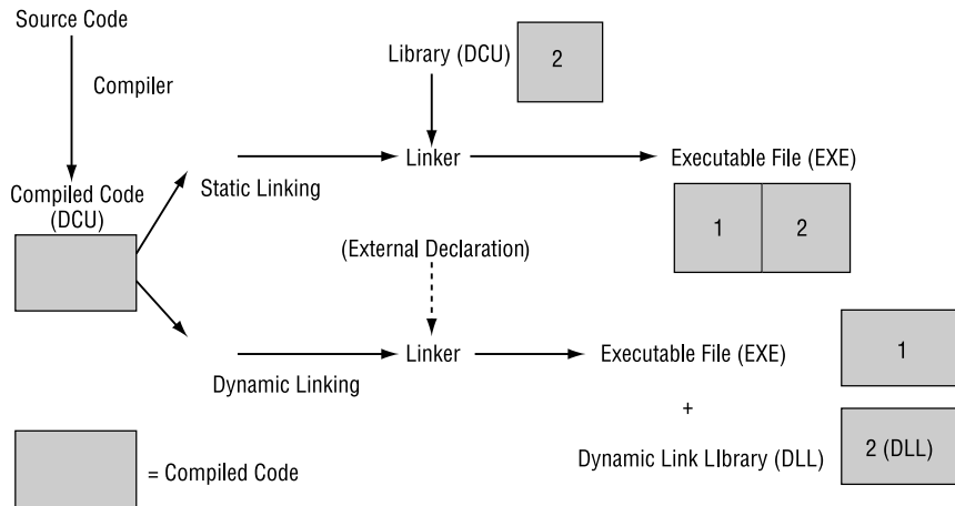
FIGURE 12.1: Static and dynamic linking in Windows
