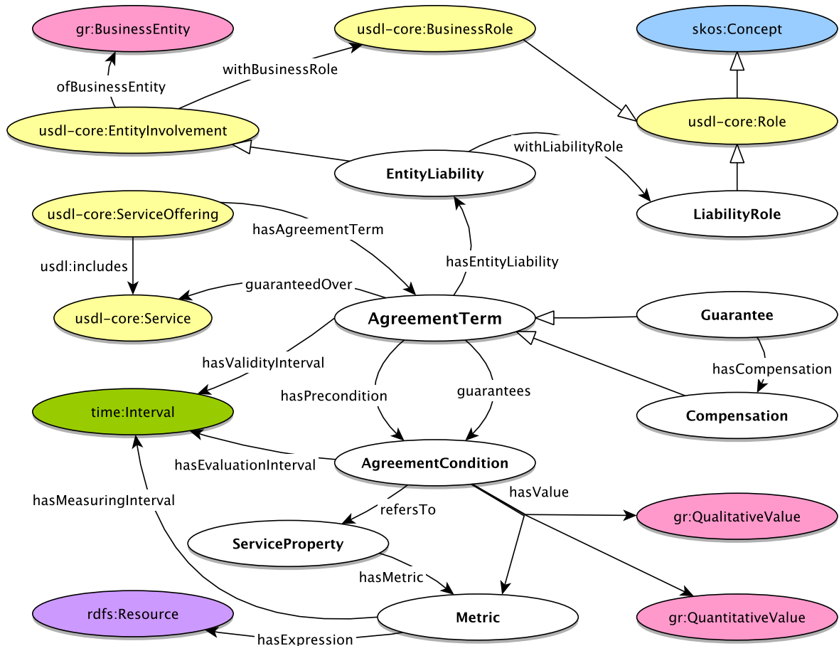
Figure 1. Linked USDL Agreement module
