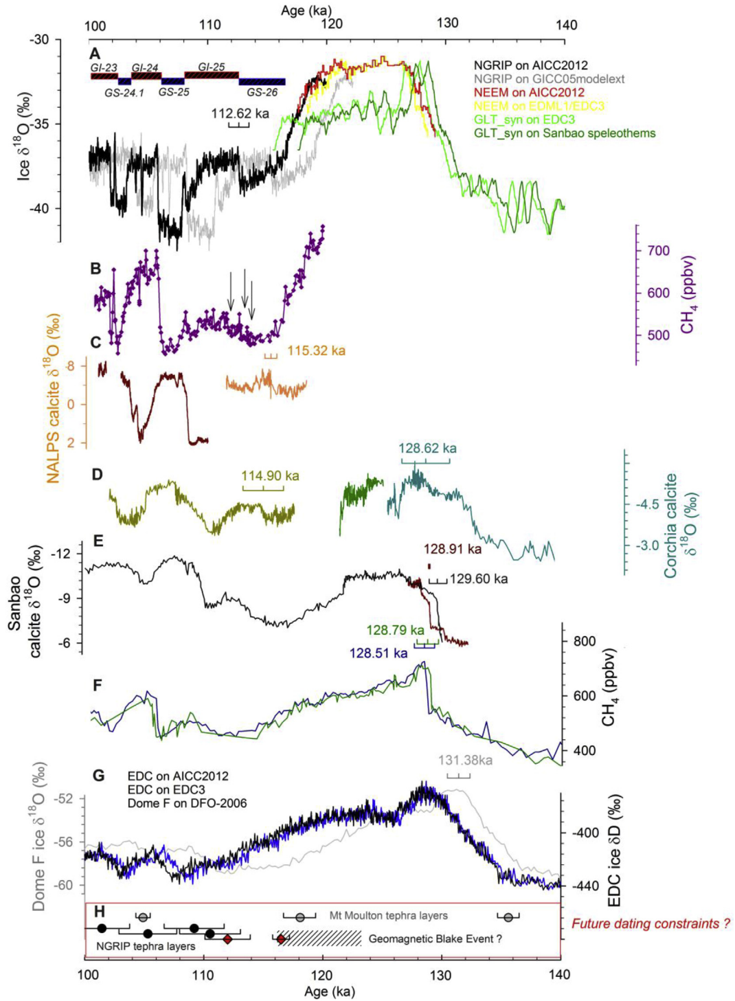
Fig. 7. From top to bottom: A. NGRIP ice \delta^{18}O (black, North Greenland Ice Core Project members, 2004) displayed on the GICC05modelext (grey) and AICC2012 (black) ice timescales, NEEM ice \delta^{18}O on the AICC2012 ice timescale (red) and on the EDML1 timescale (Ruth et al., 2007) which is by construction coherent with the EDC3 timescale (yellow) (NEEM community members, 2013), the Greenland Interstadial/Stadial (GI/GS) succession numbering follows Rasmussen et al. (2014). For higher clarity, we do not detail here the numbering of the sub-millennial scale climatic events (see Rasmussen et al., 2014 for details). B. NGRIP CH_4 concentration (purple, Capron et al., 2010; 2012) on the AICC2012 gas timescale. Arrows indicate the millennial-scale CH_4 variations occurring during GS-26 and GI-25 making difficult to define a precise CH_4 tie point with Antarctic CH_4 records. C. Calcite \delta^{18}O from NALPS speleothems (orange, Boch et al., 2011). D. Calcite \delta^{18}O from Corchia cave (light green, Drysdale et al., 2009), (dark green, Drysdale et al., 2007). E. Sanbao cave \delta^{18}O record (black, Wang et al., 2008), (brown, Cheng et al., 2009). F. Vostok (green) and EDC (blue) CH_4 records on the AICC2012 gas timescale. G. EDC \delta D (Jouzel et al., 2007) on the AICC2012 ice timescale (black, Bazin et al., 2013; Veres et al., 2013) and the EDC3 ice timescale (blue, Parrenin et al., 2007) and Dome F ice \delta^{18}O on the DFO-2006 ice timescale (grey, Kawamura et al., 2007). Dates together with associated published error bars are indicated for the penultimate deglaciation and at the onset of GI-25 (when unambiguously identified). Potential future dating constraints are indicated in H: tephra layers radiometrically dated in the Mount Moulton (grey dot, Dunbar et al., 2008) and NGRIP (black dot, Davies et al., 2014) ice cores. The location of the Blake event is indicated as deduced from orbital dating in paleosols and loess record (shaded area, Zhu et al., 1994; Fang et al., 1997; Guyodo and Valet, 1999) and as ^{40}Ar/^{39}Ar dated in speleothems from Spain (diamonds, Osete et al., 2012). See Fig. 2 for site locations.
