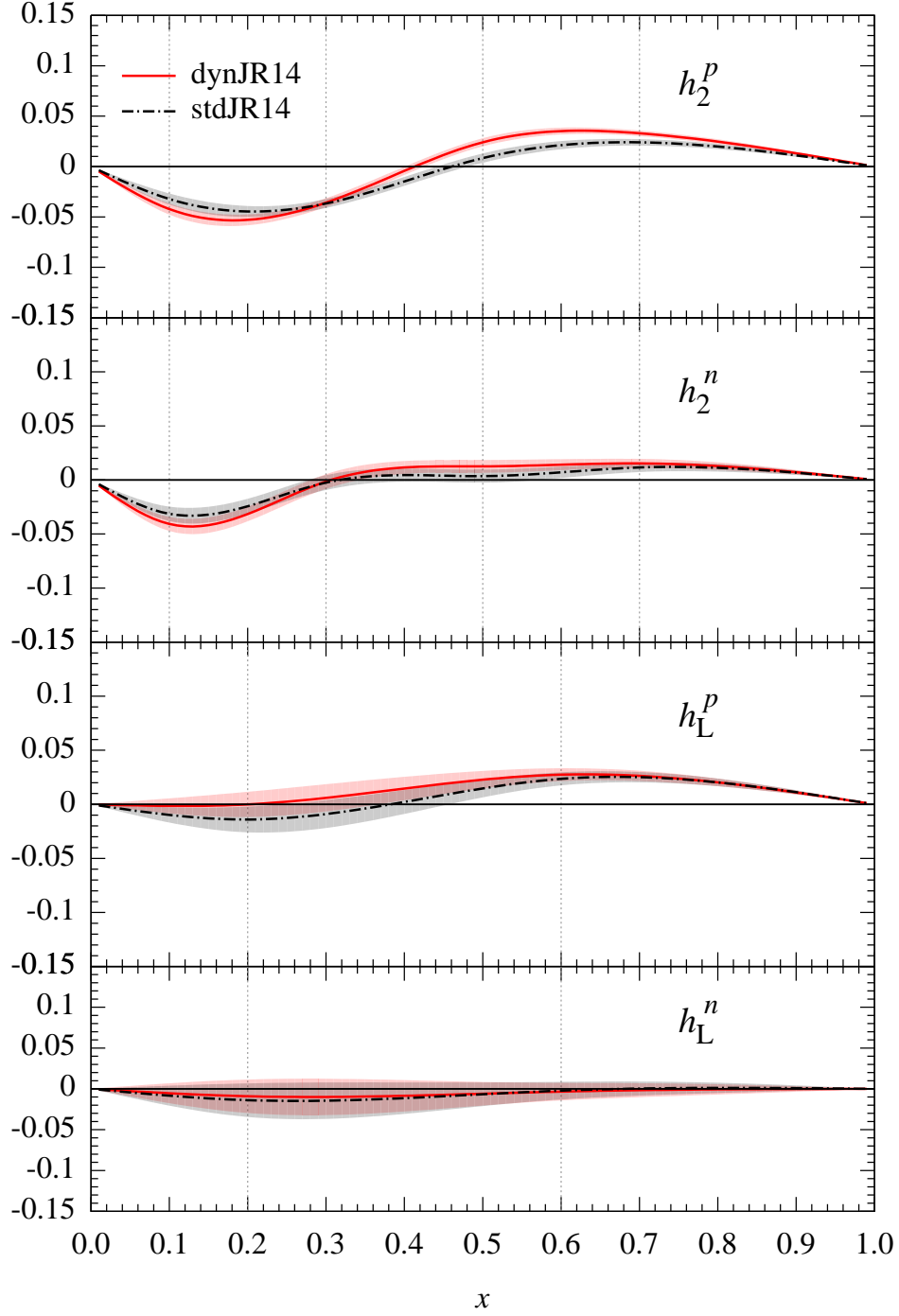
Figure 8: The central values and 1\sigma bands of the higher-twist ( \tau = 4 ) contributions (in units of \text{GeV}^2 ) to the structure functions in Eq.(3) at NNLO.
