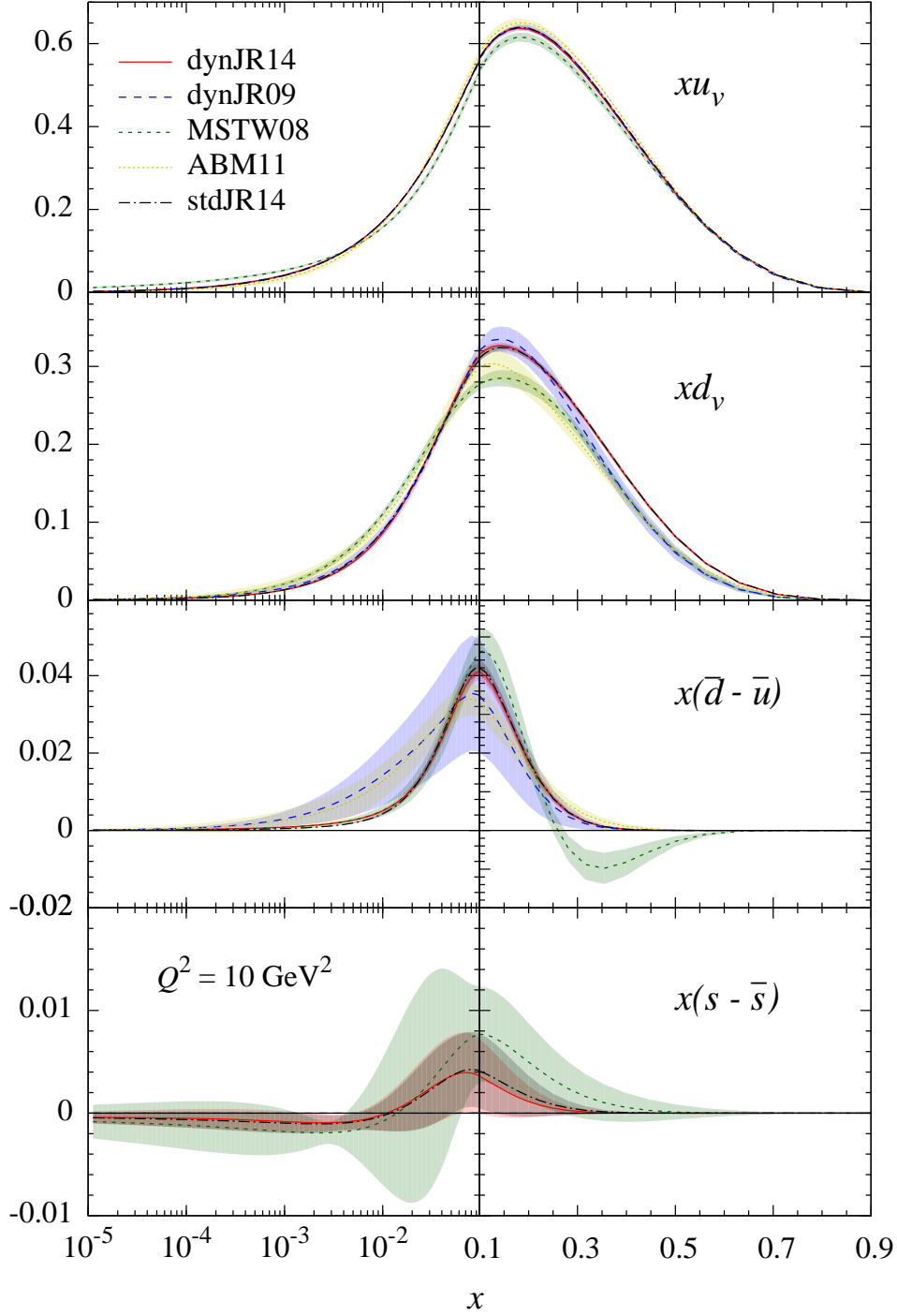
Figure 4: Non-singlet NNLO distributions at Q^2 = 10 \text{ GeV}^2 . Our present dynamical and standard PDFs are denoted by dynJR14 and stdJR14, respectively, and our previous dynamical JR09 results are taken from [2]. These results are compared with the ones of ABM11 [5] and the 3-flavor MSTW08 [56] distributions.
