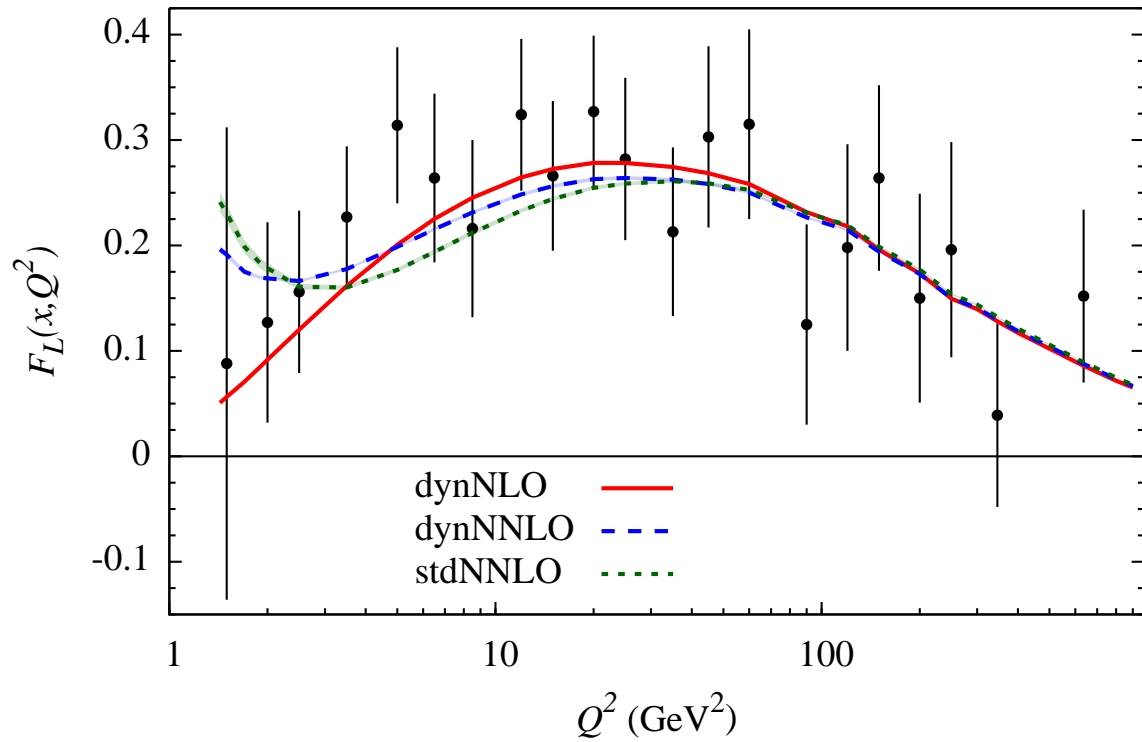
Figure 9: The dynamical and standard predictions for the longitudinal structure function F_L . The (small) 1\sigma uncertainty bands amount to only 0.5 – 1%. The data [41] cover a huge small- x domain between 3 \times 10^{-5} (small Q^2 ) and 2 \times 10^{-2} (large Q^2 ).
