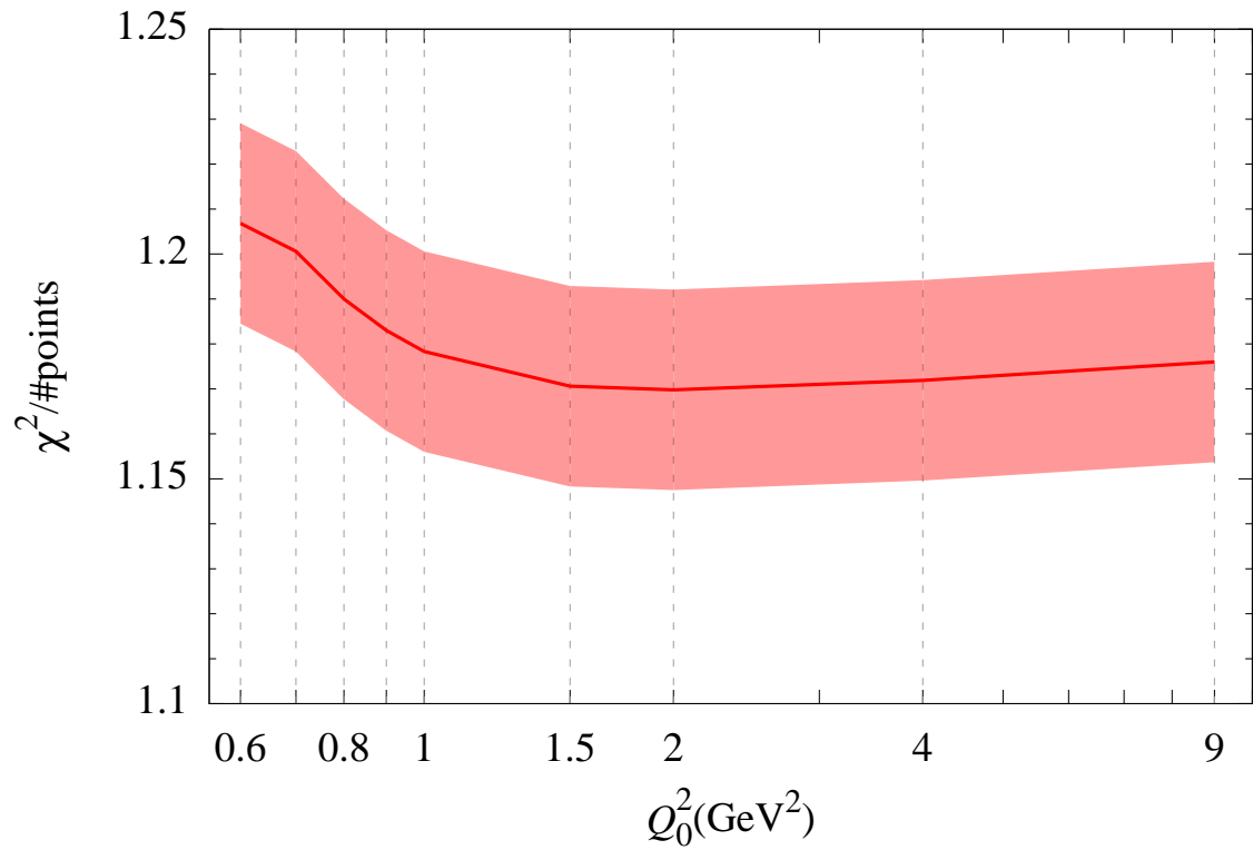
Figure 1: The dependence of \chi^2 on the variations of the input scale Q_0 as obtained in our NNLO analyses. The band indicates the \pm 1\sigma uncertainties ( \Delta\chi^2 \simeq \sqrt{2N} for N data points).
