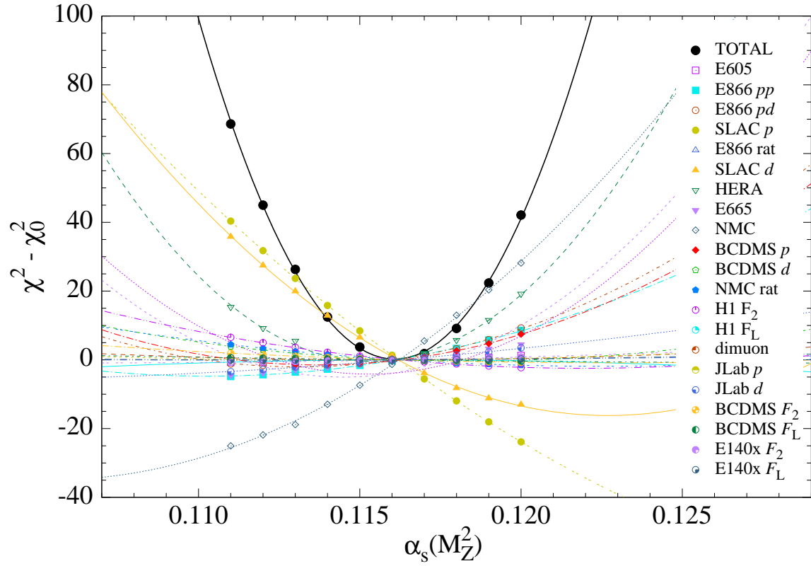
Figure 3: The dependence of \chi^2 on \alpha_s(M_Z^2) around the minimum \chi_0^2 for our standard NNLO analysis.
