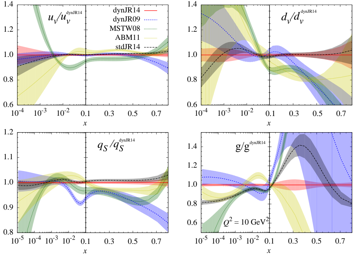
Figure 6: As in Fig. 4 but for the ratios of NNLO PDFs with respect to our present dynamical result. The fermionic singlet distribution is defined by q_S = u + \bar{u} + d + \bar{d} + s + \bar{s} .
