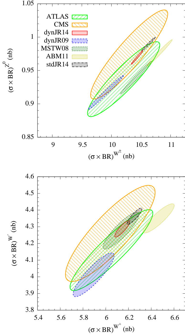
Figure 12: 1\sigma ( \Delta\chi^2 = 2.3 ) ellipses for W^\pm \equiv W^+ + W^- vs. Z^0 and W^+ vs. W^- total pp cross sections at NNLO, compared to the LHC data from ATLAS [67] and CMS [68] at \sqrt{s} = 7 TeV. For comparison we display the dynamical predictions of JR09 [3] as well as of ABM11 [5] and MSTW08 [1].
