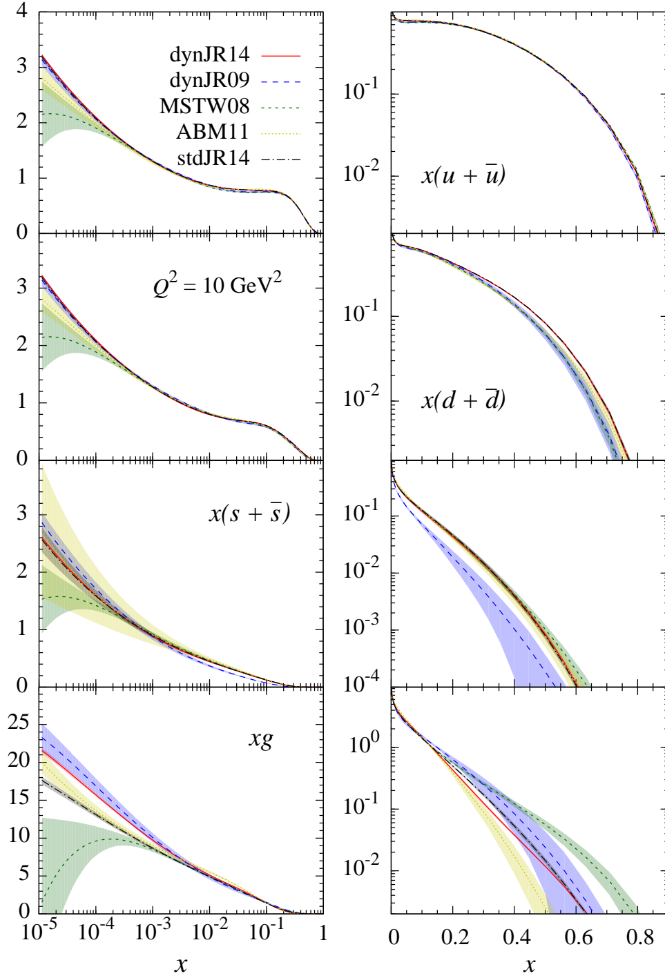
Figure 5: As in Fig. 4 but for the singlet sector.
