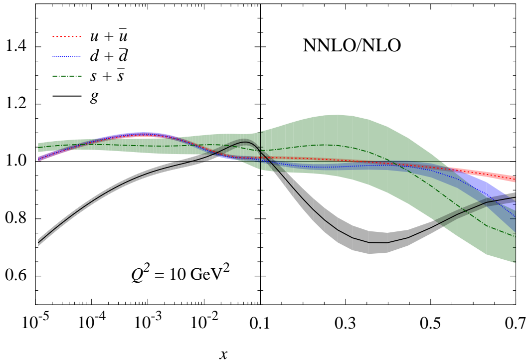
Figure 7: The NNLO/NLO ratios of our dynamical JR14 parton distributions.
