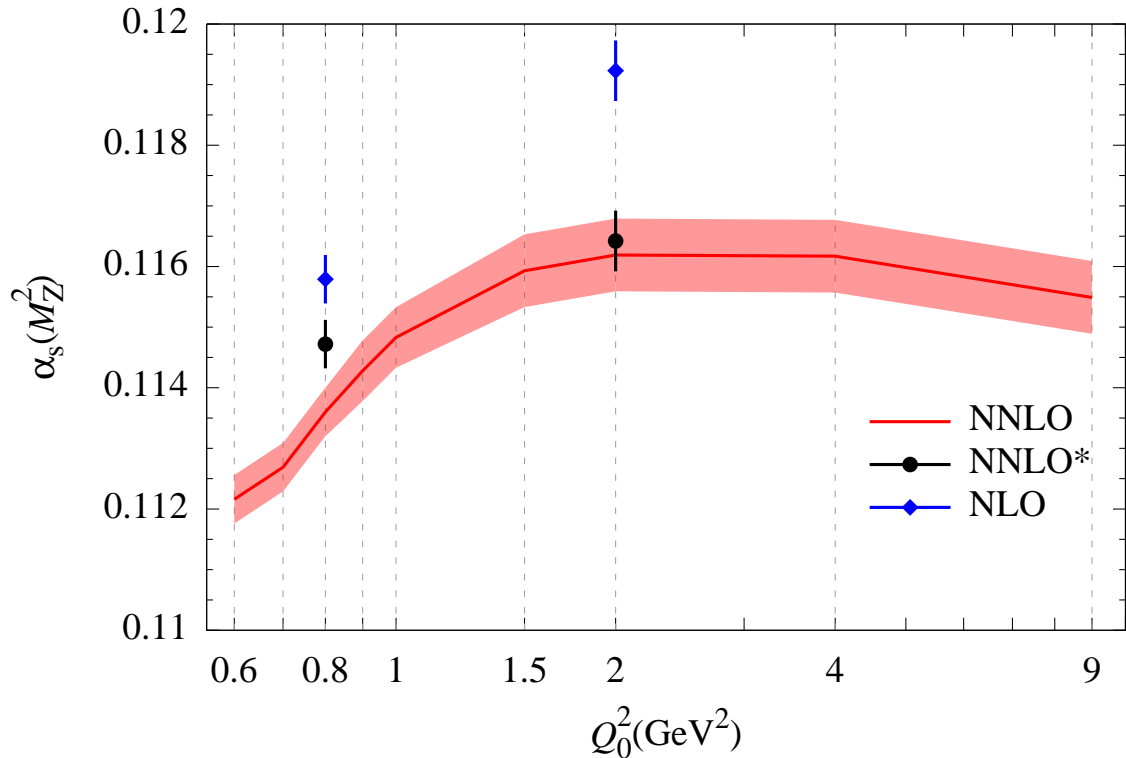
Figure 2: The dependence of \alpha_s(M_Z^2) on the variations of the input scale Q_0 as obtained in our NNLO analyses, together with the 1\sigma uncertainty band ( \Delta\chi^2 = 1 ). For illustration we show the sensitivity of two of our results when including jet and charm data at NNLO as well, denoted by NNLO*, where NLO matrix elements have been (inconsistently) combined with NNLO PDFs. The NLO results at the input scales 0.8 \text{ GeV}^2 (dynamical) and 2 \text{ GeV}^2 (standard) are depicted as well.
