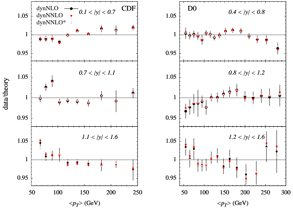
Figure 11: Comparison of Tevatron hadronic jet-data [48, 49] with consistent theoretical dynamical NLO results, and (inconsistent) NNLO expectations: NNLO* refers to fitting NNLO PDFs using NLO matrix elements, and NNLO uses our optimal fixed NNLO PDFs (no fit) together with NLO matrix elements.
