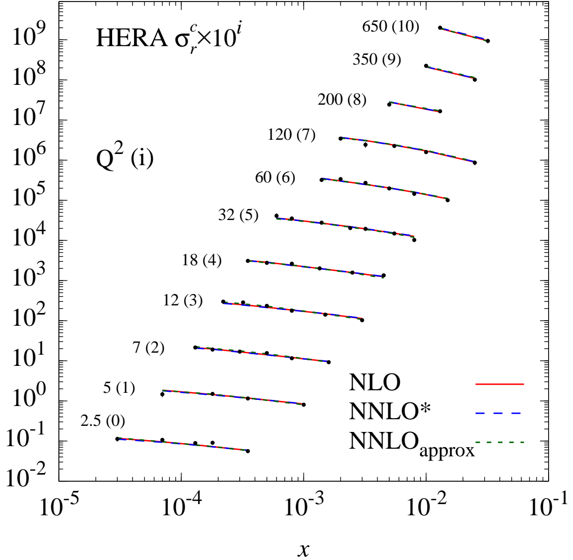
Figure 10: Theoretical NLO predictions and NNLO expectations for DIS charm production at fixed values of Q^2 (GeV 2 units). NNLO* refers to NNLO fits using (incorrectly) massive NLO sub-cross sections. The optimal approximate NNLO approx expectations are described in the text. The shifts r_j induced by the systematic errors (cf. Eq.(5)) are included in the theoretical predictions, and the errors shown are only statistical. The HERA ‘reduced’ cross-section data are taken from [40].
