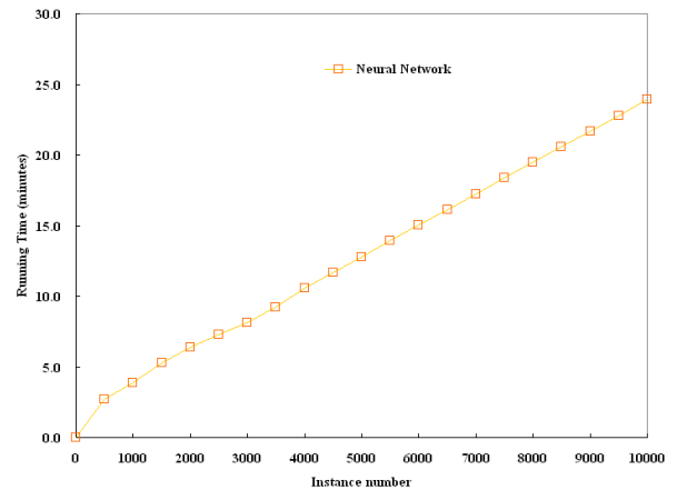
Figure 6. Instance number vs running time by back-propagation neural network
