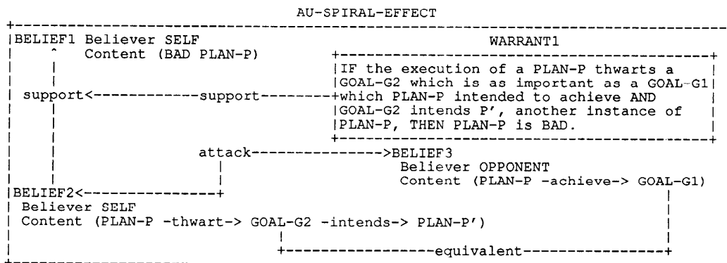
Figure 4. AU-SPIRAL-EFFECT
