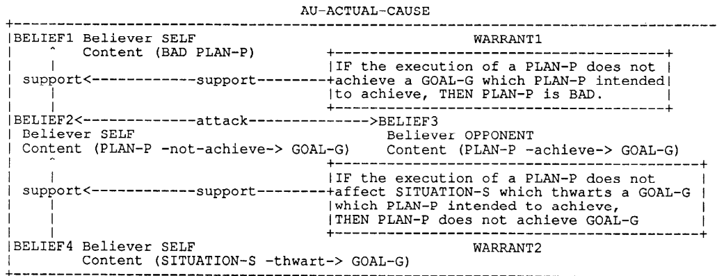
Figure 1. AU-ACTUAL-CAUSE
