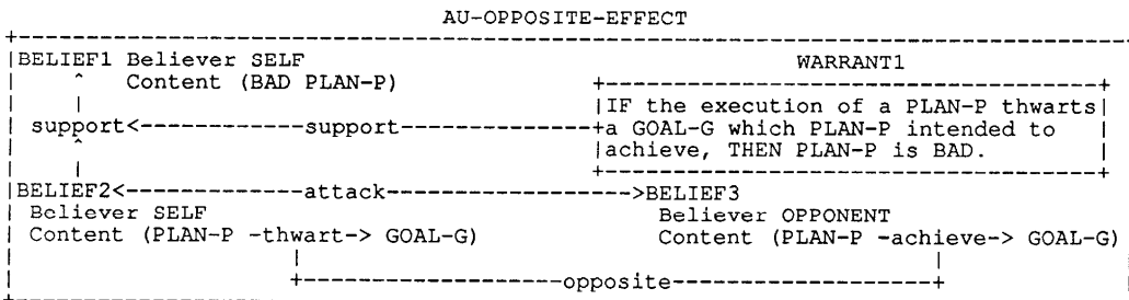
Figure 2. AU-OPPOSITE-EFFECT
