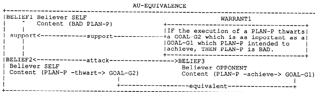
Figure 3. AU-EQUIVALENCE
