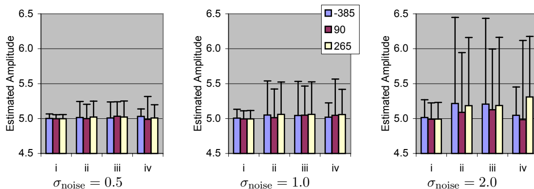
Fig. 6. Graphical presentation of the results in Table I.
