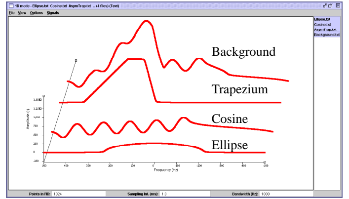
Fig. 2. Spectrum of a simulated macromole signal – background – using the four basic shapes shown in Fig. 1. First, a trapezium was made from a rectangle and two right-angled triangles. Next, an ellipse was added. Each was broadened and shifted by multiplication in the time domain with an appropriate exponential \exp[-\alpha t - (\beta t)^2 + i\omega t] . Finally, a series of five connected cosines was added to produce undulations. The phase of the cosines was rotated by 90 deg to augment the complexity.
