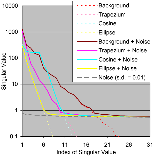
Fig. 3. Singular values of L=512 by M=513 Hankel matrices formed from the signals corresponding to the trapezium, ellipse, and cosine-series, and their sum, shown in Fig. 1, for one level of added noise. N = 1024 .
