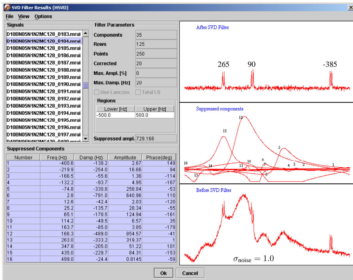
Fig. 5. Background removal by HSVD. Bottom-right: Three metabolite doublets superimposed on the broad background shown in Fig. 2. Middle-right: HSVD-parameterized background comprising 16 components. Upper-right: Difference between the previous two, showing clearly the three metabolite doublets, at 265 Hz, 90 Hz, and -385 Hz. The amplitudes and damping factors of all doublet components are 5.0 (in arbitrary units) and 10 Hz, respectively.
