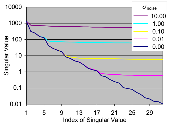
Fig. 4. Singular values of an L=512 by M=513 Hankel matrix formed from the signal corresponding to the background spectrum shown in Fig. 1, for five levels of added noise. N = 1024 . Reduction of L and M by a factor of four, using only the first L + M - 1 samples, reduces the effect of noise significantly.
