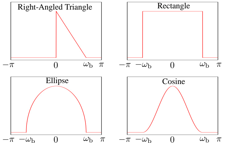
Fig. 1. Frequency-domain presentation of the four elementary shapes used for designing background spectra. Clock-wise, starting upper left: right-angled triangle, rectangle, ellipse, cosine. See also the formulae in the text. The triangle can be reflected with respect to \omega = 0 by changing the sign of \omega_b .
