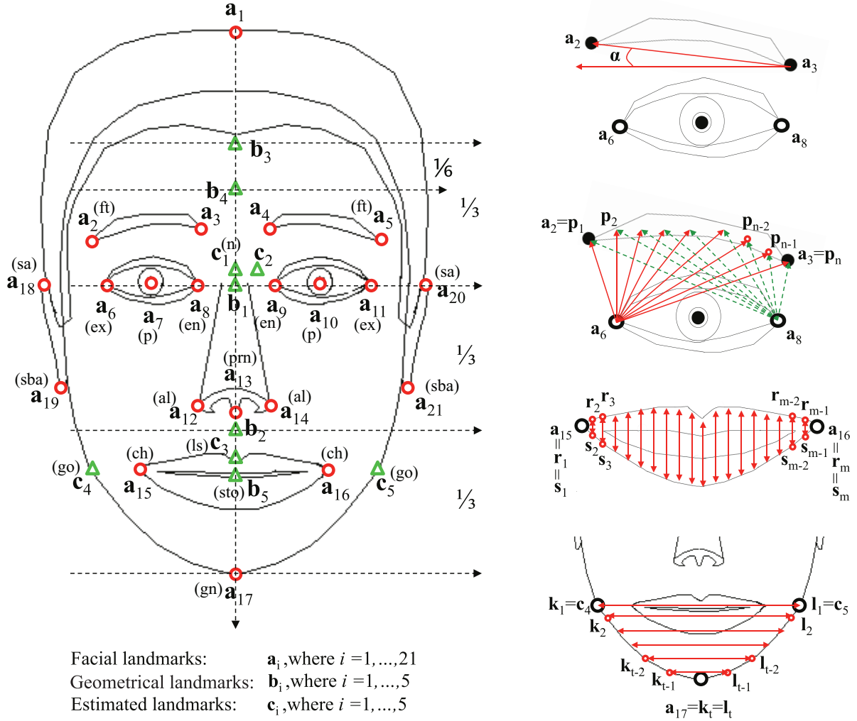
Figure 2: Left: Face layout with landmarks: facial ( a_i ), geometrical ( b_i ) and estimated ( c_i ). Right: Visual representation of distances calculation between landmarks for computing the soft features (see Table 1). Standard anthropometric landmarks names [37] are given in brackets next to the corresponding landmarks used in this study.
