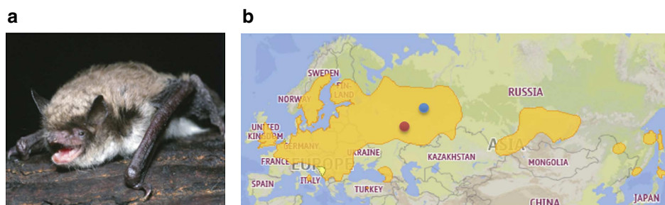
Figure 1 | Species map of M. brandtii . (a) M. brandtii . (b) Occurrence of M. brandtii and areas of sample collection. Coloured dots indicate the location of sampled hibernating (December and April; shown in blue) and summer-active (June; shown in red) animals.
