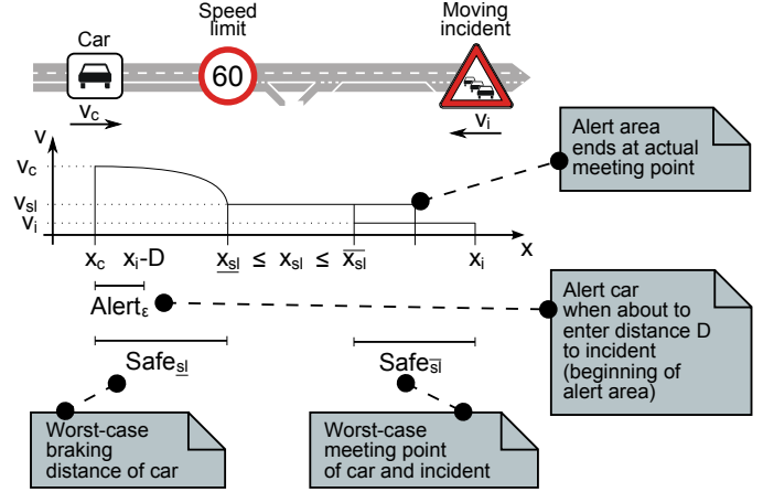
Fig. 1. Speed limit control in presence of a moving incident
