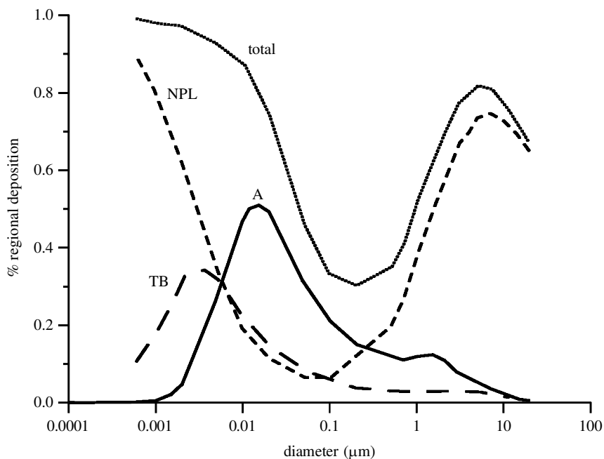
Figure 6. Predicted deposition of inhaled particles of different sizes of unit density in the human respiratory tract during nose breathing, light exercise (ICRP 1994). ‘NPL’ denotes nasopharyngolaryngeal deposition; ‘TB’ denotes tracheobronchial deposition; ‘A’ denotes alveolar deposition; ‘total’ denotes the sum of particle depositions in the respiratory tract for all three compartments.
