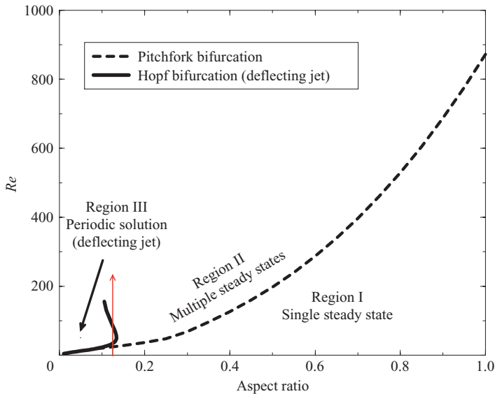
FIGURE 10. Map of the parameter space indicating different flow regimes arising in planar counterflowing jets. The red arrow indicates the continuation path used to construct the bifurcation diagram shown in figure 11.
