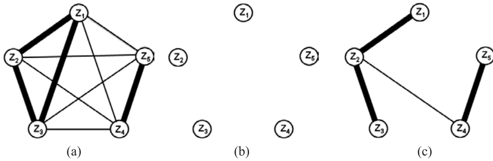
Fig. 1. (a) Graphical model of the underlying distribution P(Z) . Mutual information between variables is shown by the thickness of the edge. (b) Naive Bayes approximation. (c) Chow Liu tree.
