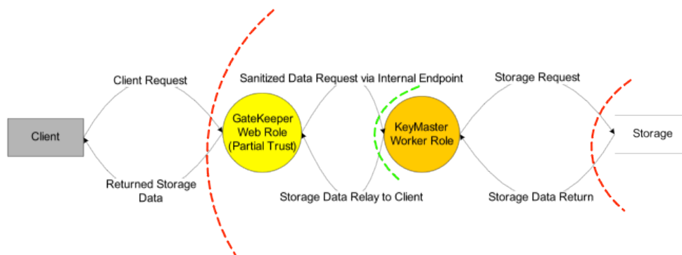
Figure 1: The Gatekeeper Design Pattern
