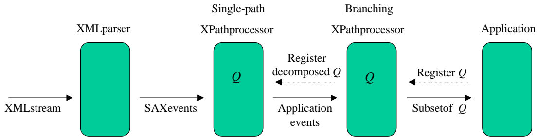
Figure 3: System Architecture
