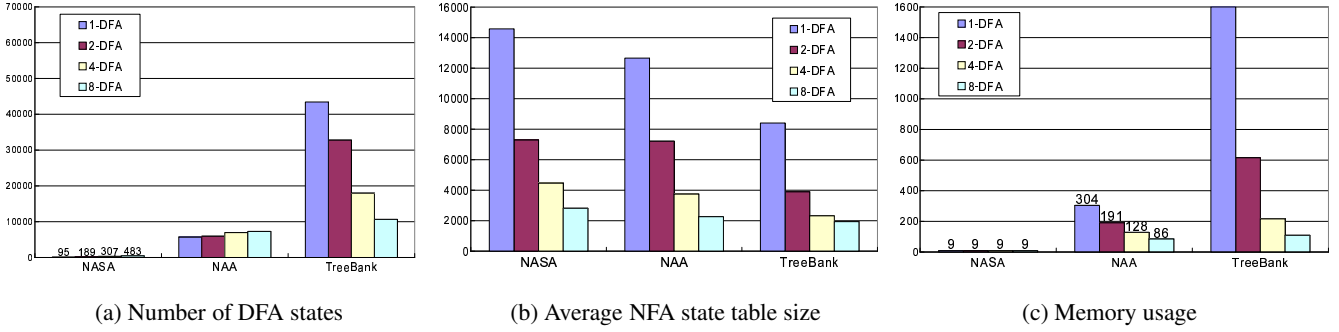
Figure 8: Evaluations of n -DFA; XPEs 100K, \text{prob}(//) 5%, \text{prob}^* 5%
