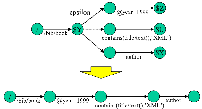
Figure 6: An example of optimized NFA conversion
