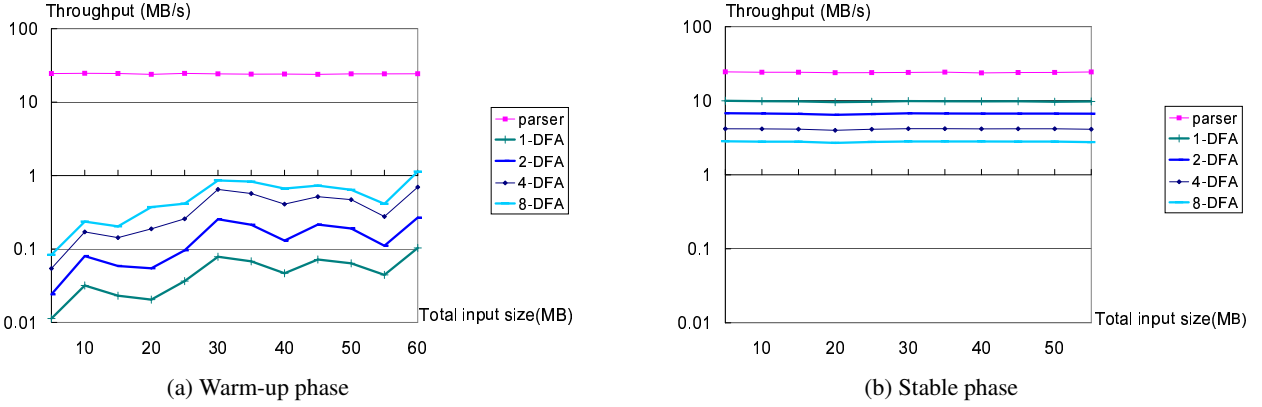
Figure 10: Throughput Experiments for n-DFA (n = 1,2,4,8)
