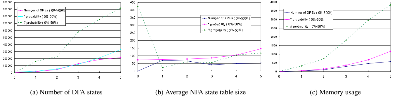
Figure 11: Evaluations of 8-DFA with Shared NFA state table technique: TreeBank XML
