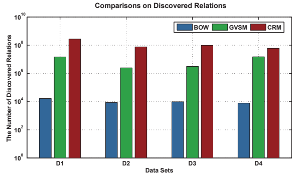
Fig. 6. Comparisons of the number of discovered relations on four data sets.
