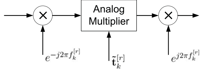
Fig. 2. The baseband processing structure at the relays for the case of AF relaying multi-relay networks ( f_k^{[r]} denotes the carrier frequency at the k th relay).
