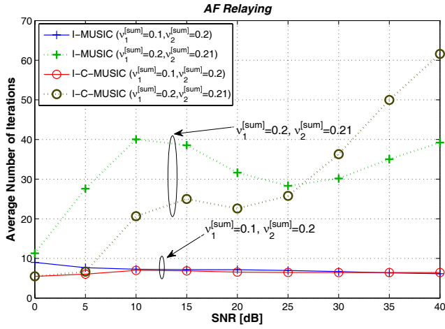
Fig. 7. Average number of iterations for I-MUSIC and I-C-MUSIC for the estimation of v_1^{[\text{sum}]} for AF networks with L = 24 and L_F = 512 .
