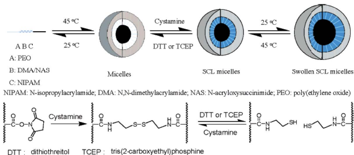
Fig. 3 Schematic illustration of the formation of reversible shell cross-linked micelles from PEO- b -(DMA- s -NAS)- b -NIPAM triblock copolymers. (Reproduced with permission from Ref. 16. Copyright 2006 American Chemical Society.)
