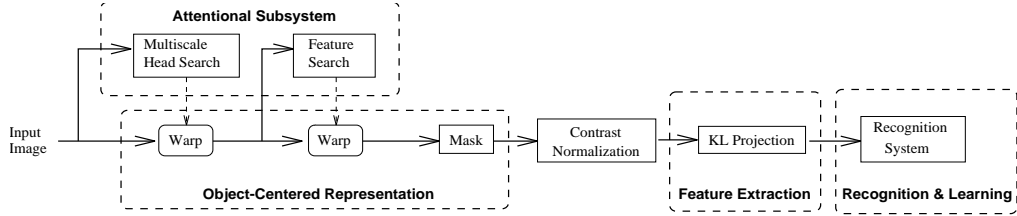
Figure 6: The face processing system.
