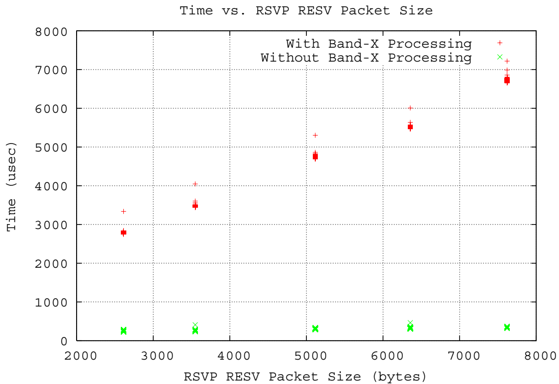
Figure 11. Times elapsed between receiving and forwarding of RSVP RESV packets. All measurements taken at a single node along the reservation path. One hundred samples were taken for each size. The machine was a Dell PowerEdge 1550.
