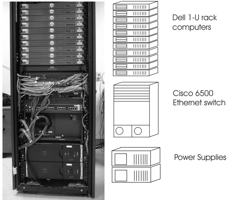
Figure 9. The equipment used to implement the network testbed.
