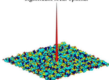
Fig. 6. Functions whose global structure provides no useful information about its optima.
