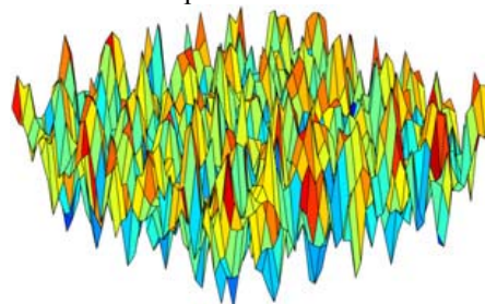
Fig. 4. Functions with a huge number of significant local optima.
