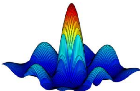
Fig. 5. Functions with a small number of significant local optima.
